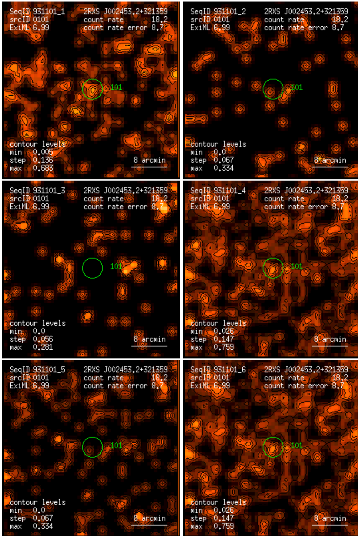
Figure 101: RASS 931101: detection 0101: band rate images, Gaussian filter: (1) PSPC channels 11 – 41, (2) 52 – 90, (3) 91 – 201, (4) 11 – 235, (5) 52 – 201, (6) 11 – 201. Broad band rates in counts/ks. Band rate contour levels in counts/ks/arcmin 2 .
