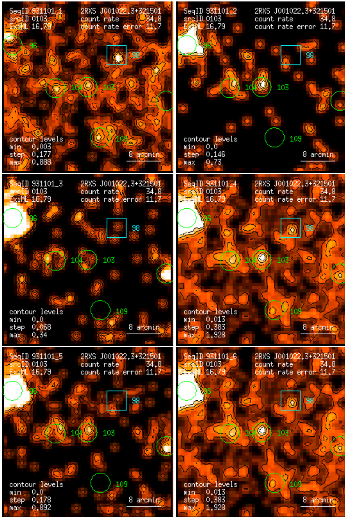
Figure 103: RASS 931101: detection 0103: band rate images, Gaussian filter: (1) PSPC channels 11 – 41, (2) 52 – 90, (3) 91 – 201, (4) 11 – 235, (5) 52 – 201, (6) 11 – 201. Broad band rates in counts/ks. Band rate contour levels in counts/ks/arcmin 2 .
