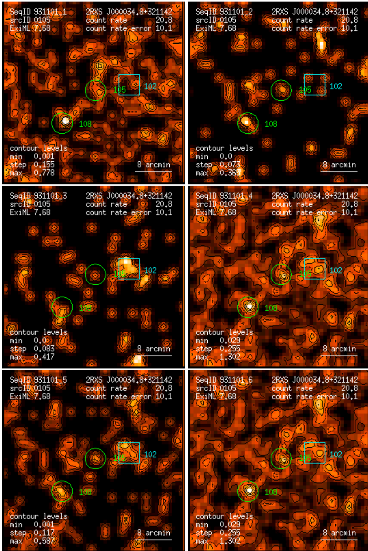
Figure 105: RASS 931101: detection 0105: band rate images, Gaussian filter: (1) PSPC channels 11 – 41, (2) 52 – 90, (3) 91 – 201, (4) 11 – 235, (5) 52 – 201, (6) 11 – 201. Broad band rates in counts/ks. Band rate contour levels in counts/ks/arcmin 2 .
