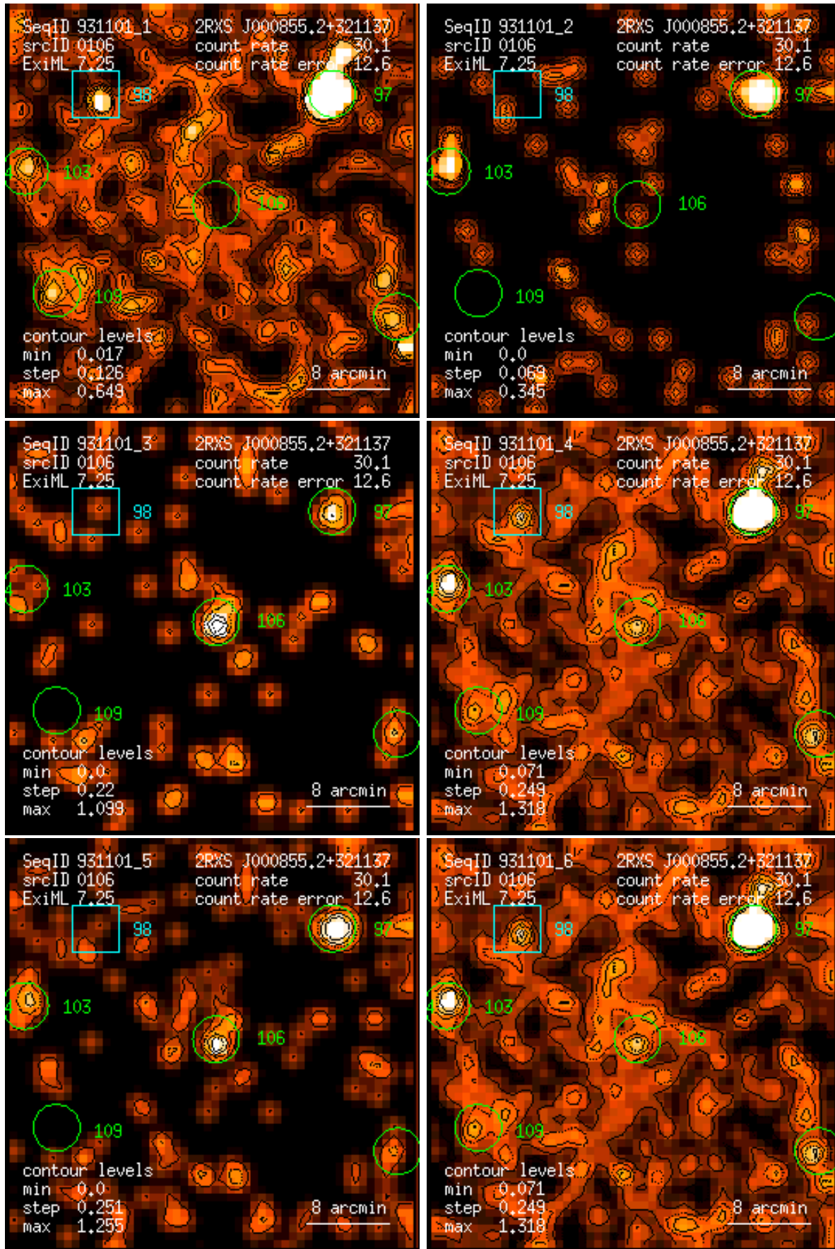
Figure 106: RASS 931101: detection 0106: band rate images, Gaussian filter: (1) PSPC channels 11 – 41, (2) 52 – 90, (3) 91 – 201, (4) 11 – 235, (5) 52 – 201, (6) 11 – 201. Broad band rates in counts/ks. Band rate contour levels in counts/ks/arcmin 2 .
