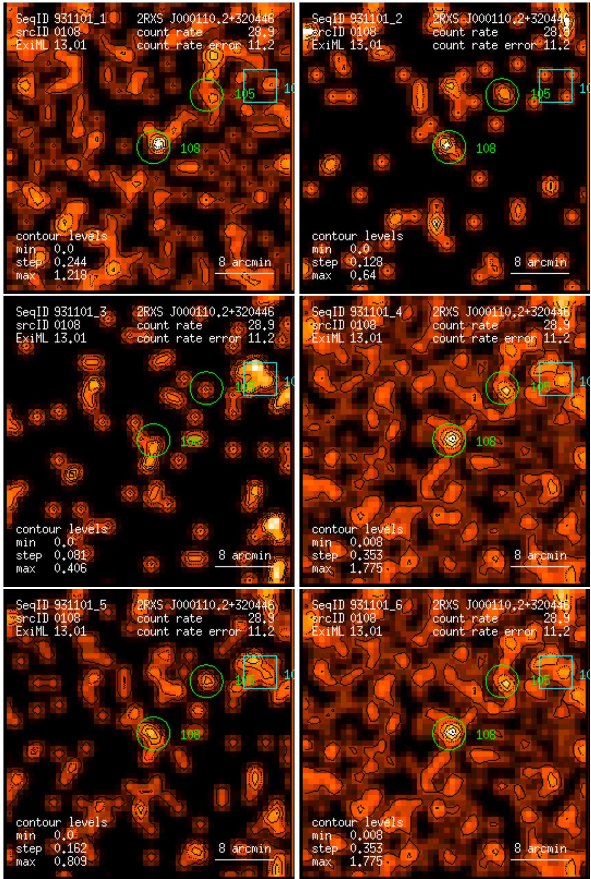
Figure 108: RASS 931101: detection 0108: band rate images, Gaussian filter: (1) PSPC channels 11 – 41, (2) 52 – 90, (3) 91 – 201, (4) 11 – 235, (5) 52 – 201, (6) 11 – 201. Broad band rates in counts/ks. Band rate contour levels in counts/ks/arcmin 2 .
