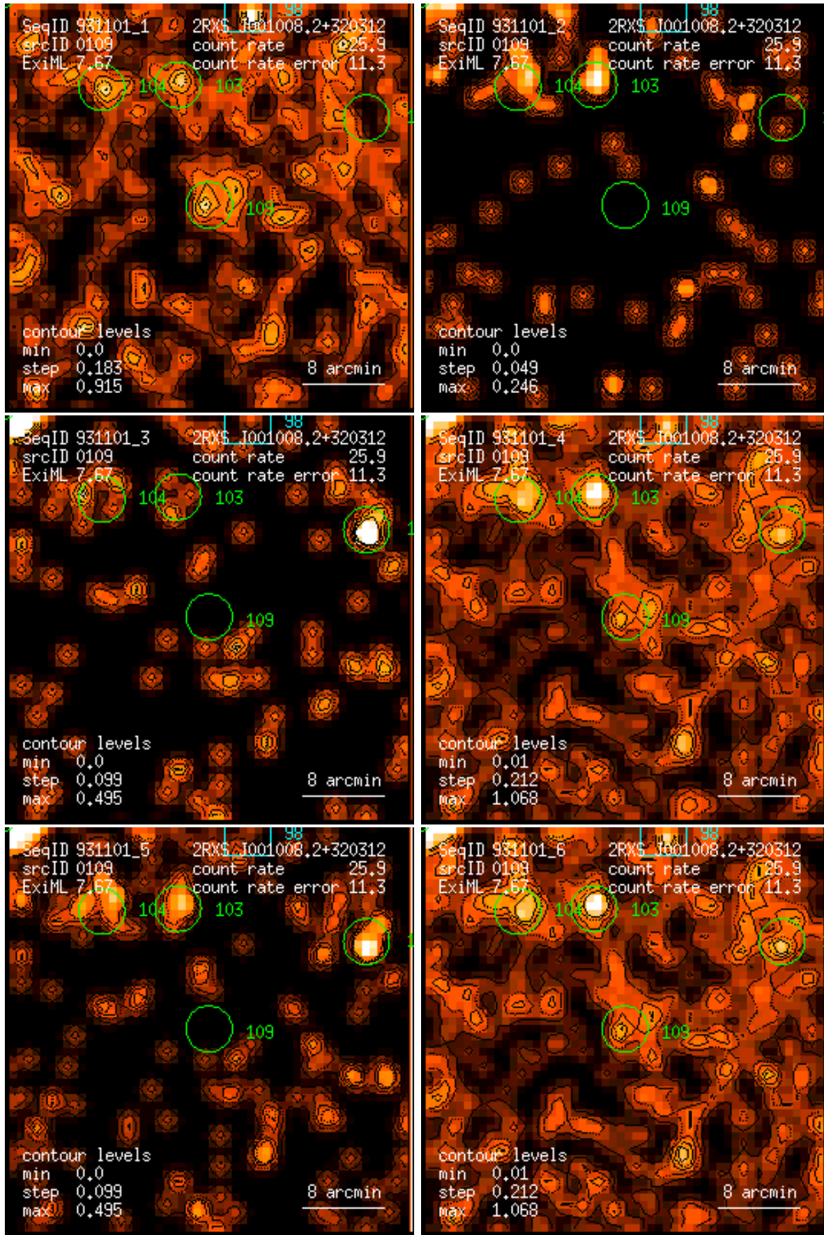
Figure 109: RASS 931101: detection 0109: band rate images, Gaussian filter: (1) PSPC channels 11 – 41, (2) 52 – 90, (3) 91 – 201, (4) 11 – 235, (5) 52 – 201, (6) 11 – 201. Broad band rates in counts/ks. Band rate contour levels in counts/ks/arcmin 2 .
