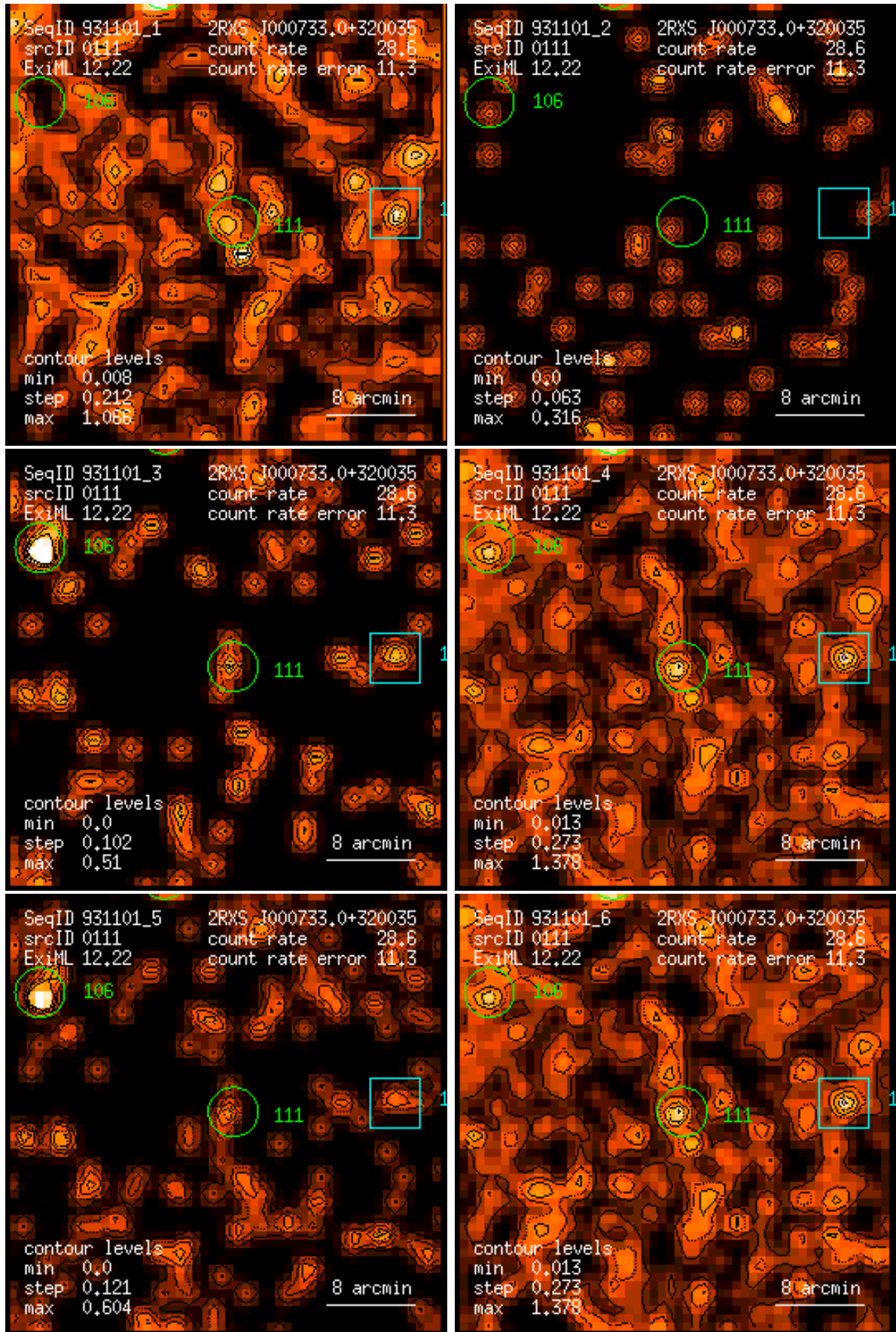
Figure 111: RASS 931101: detection 0111: band rate images, Gaussian filter: (1) PSPC channels 11 – 41, (2) 52 – 90, (3) 91 – 201, (4) 11 – 235, (5) 52 – 201, (6) 11 – 201. Broad band rates in counts/ks. Band rate contour levels in counts/ks/arcmin 2 .
