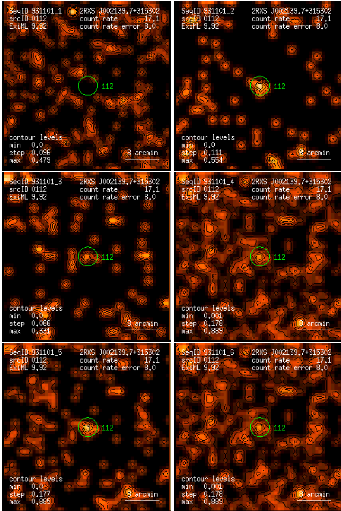
Figure 112: RASS 931101: detection 0112: band rate images, Gaussian filter: (1) PSPC channels 11 – 41, (2) 52 – 90, (3) 91 – 201, (4) 11 – 235, (5) 52 – 201, (6) 11 – 201. Broad band rates in counts/ks. Band rate contour levels in counts/ks/arcmin 2 .
