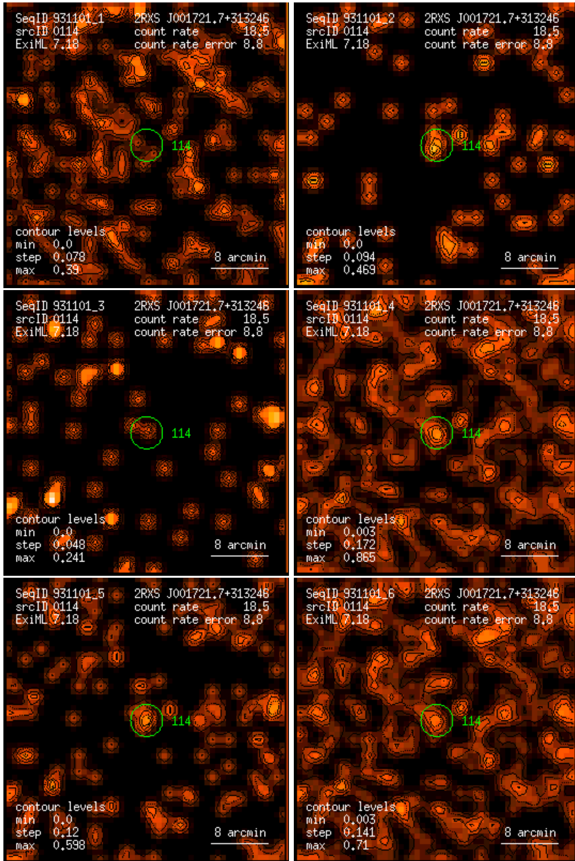
Figure 114: RASS 931101: detection 0114: band rate images, Gaussian filter: (1) PSPC channels 11 – 41, (2) 52 – 90, (3) 91 – 201, (4) 11 – 235, (5) 52 – 201, (6) 11 – 201. Broad band rates in counts/ks. Band rate contour levels in counts/ks/arcmin 2 .
