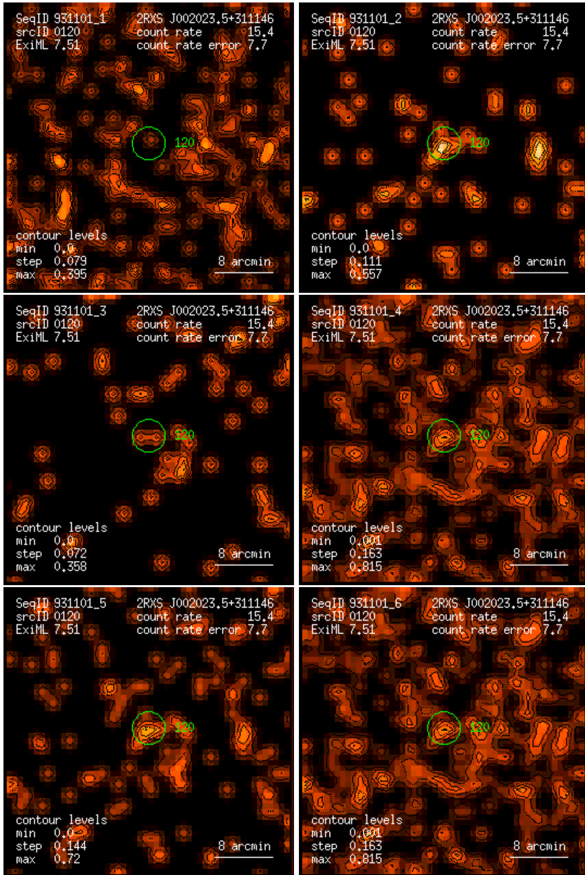
Figure 120: RASS 931101: detection 0120: band rate images, Gaussian filter: (1) PSPC channels 11 – 41, (2) 52 – 90, (3) 91 – 201, (4) 11 – 235, (5) 52 – 201, (6) 11 – 201. Broad band rates in counts/ks. Band rate contour levels in counts/ks/arcmin 2 .
