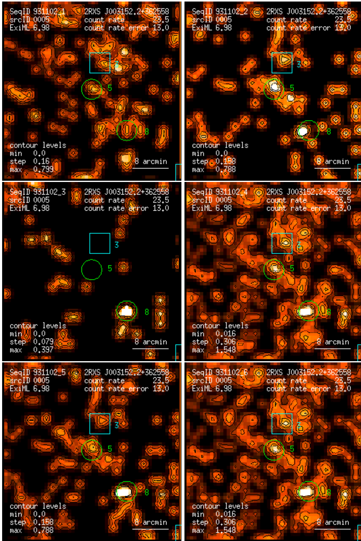
Figure 5: RASS 931102: detection 0005: band rate images, Gaussian filter: (1) PSPC channels 11 – 41, (2) 52 – 90, (3) 91 – 201, (4) 11 – 235, (5) 52 – 201, (6) 11 – 201. Broad band rates in counts/ks. Band rate contour levels in counts/ks/arcmin 2 .
