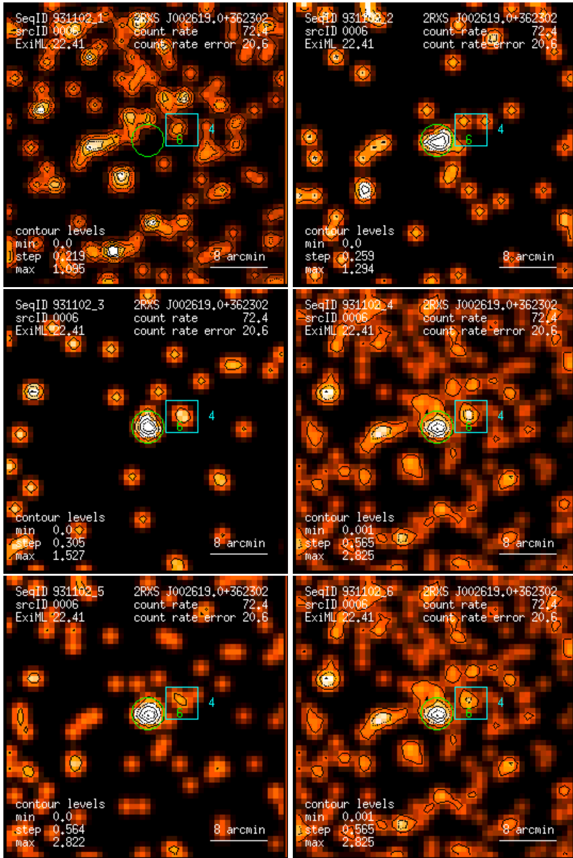
Figure 6: RASS 931102: detection 0006: band rate images, Gaussian filter: (1) PSPC channels 11 – 41, (2) 52 – 90, (3) 91 – 201, (4) 11 – 235, (5) 52 – 201, (6) 11 – 201. Broad band rates in counts/ks. Band rate contour levels in counts/ks/arcmin 2 .
