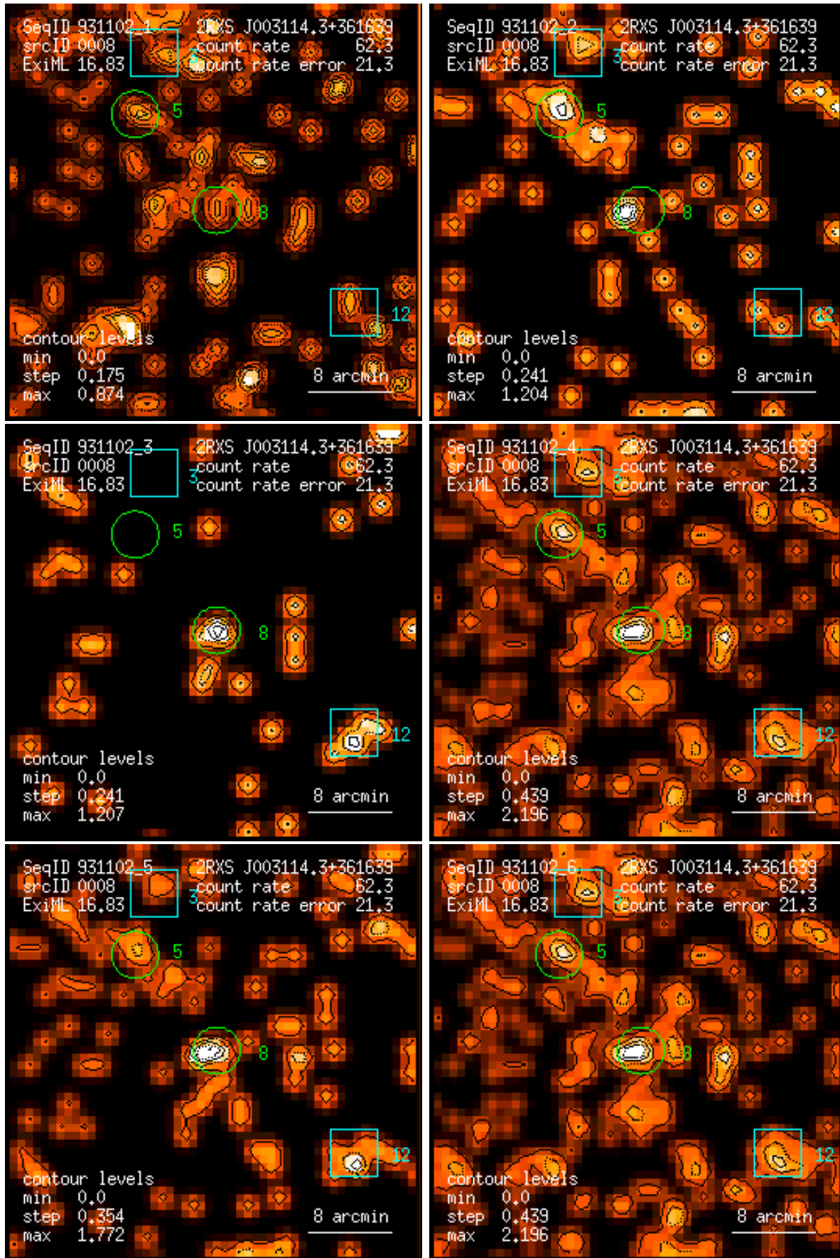
Figure 8: RASS 931102: detection 0008: band rate images, Gaussian filter: (1) PSPC channels 11 – 41, (2) 52 – 90, (3) 91 – 201, (4) 11 – 235, (5) 52 – 201, (6) 11 – 201. Broad band rates in counts/ks. Band rate contour levels in counts/ks/arcmin 2 .
