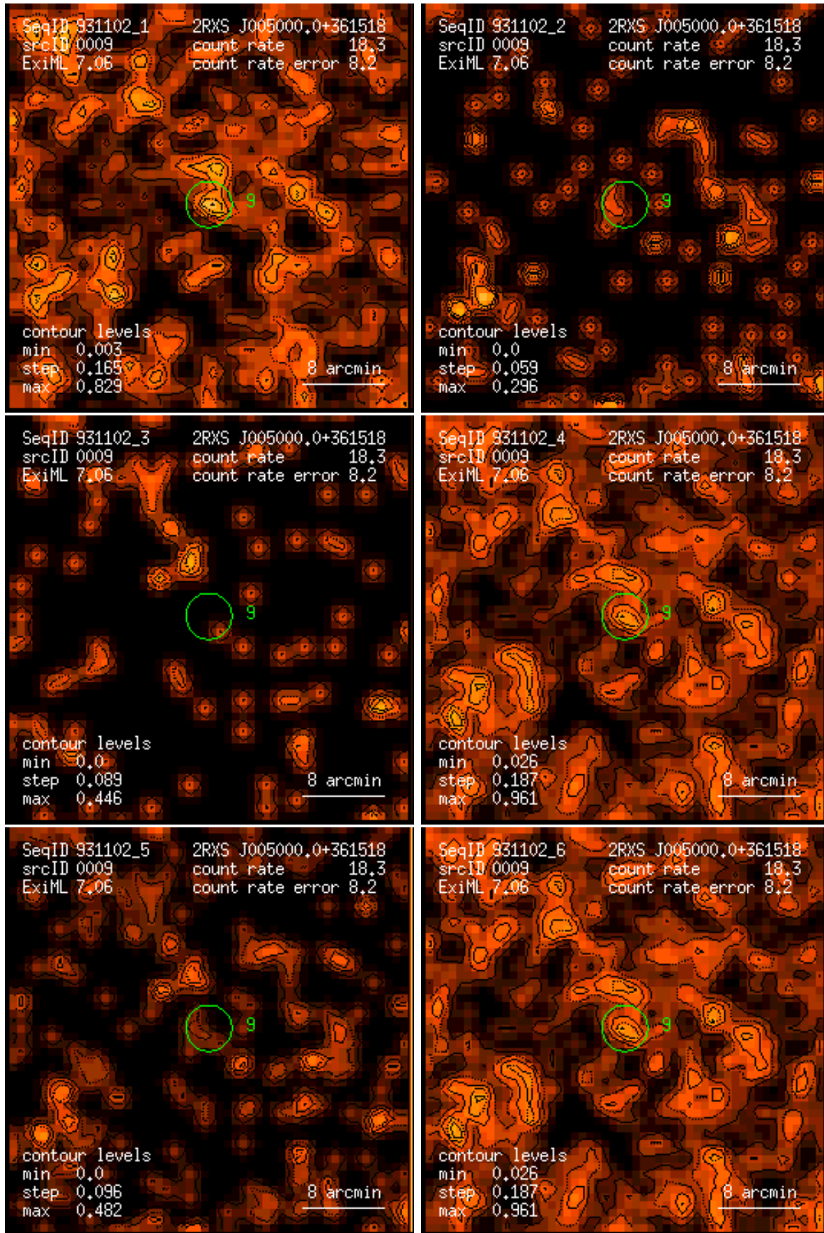
Figure 9: RASS 931102: detection 0009: band rate images, Gaussian filter: (1) PSPC channels 11 – 41, (2) 52 – 90, (3) 91 – 201, (4) 11 – 235, (5) 52 – 201, (6) 11 – 201. Broad band rates in counts/ks. Band rate contour levels in counts/ks/arcmin 2 .
