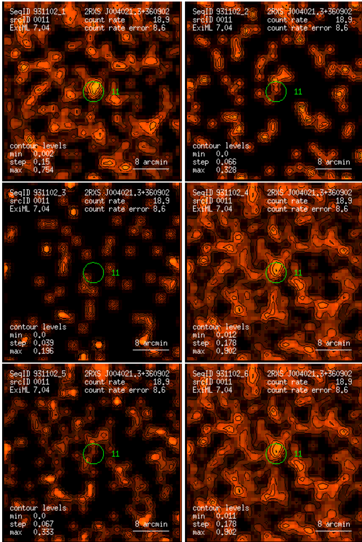
Figure 11: RASS 931102: detection 0011: band rate images, Gaussian filter: (1) PSPC channels 11 – 41, (2) 52 – 90, (3) 91 – 201, (4) 11 – 235, (5) 52 – 201, (6) 11 – 201. Broad band rates in counts/ks. Band rate contour levels in counts/ks/arcmin 2 .
