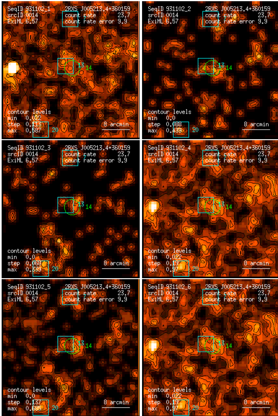
Figure 14: RASS 931102: detection 0014: band rate images, Gaussian filter: (1) PSPC channels 11 – 41, (2) 52 – 90, (3) 91 – 201, (4) 11 – 235, (5) 52 – 201, (6) 11 – 201. Broad band rates in counts/ks. Band rate contour levels in counts/ks/arcmin 2 .
