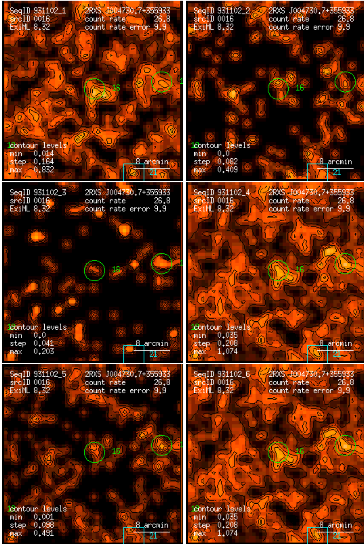
Figure 16: RASS 931102: detection 0016: band rate images, Gaussian filter: (1) PSPC channels 11 – 41, (2) 52 – 90, (3) 91 – 201, (4) 11 – 235, (5) 52 – 201, (6) 11 – 201. Broad band rates in counts/ks. Band rate contour levels in counts/ks/arcmin 2 .
