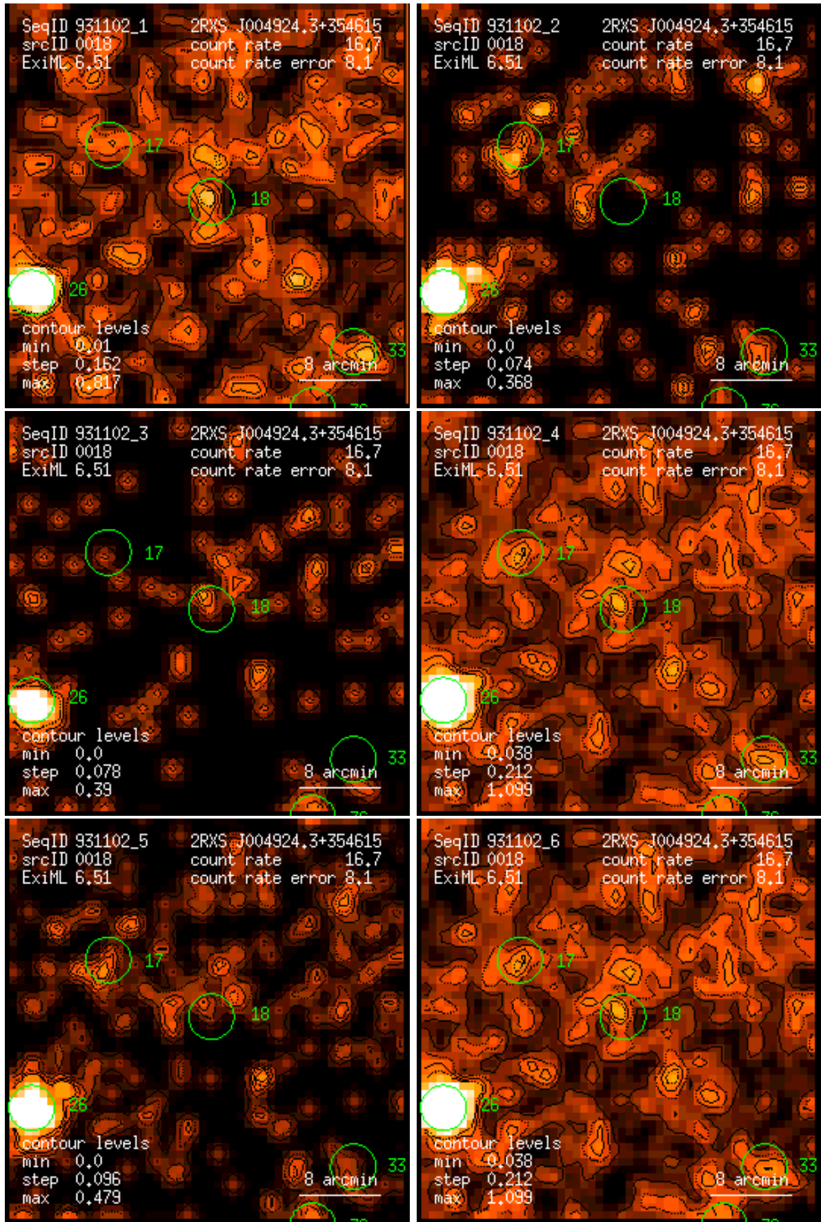
Figure 18: RASS 931102: detection 0018: band rate images, Gaussian filter: (1) PSPC channels 11 – 41, (2) 52 – 90, (3) 91 – 201, (4) 11 – 235, (5) 52 – 201, (6) 11 – 201. Broad band rates in counts/ks. Band rate contour levels in counts/ks/arcmin 2 .
