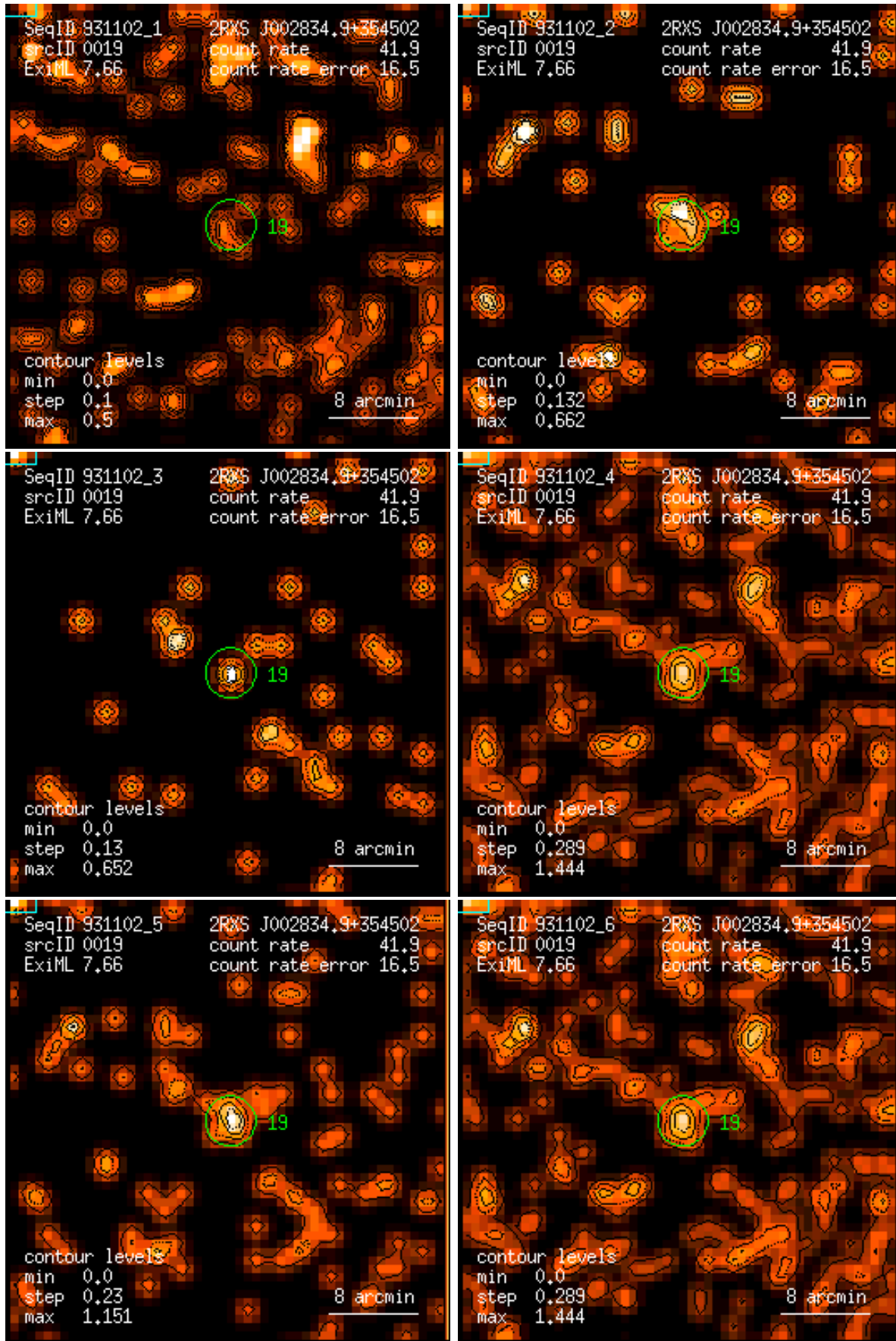
Figure 19: RASS 931102: detection 0019: band rate images, Gaussian filter: (1) PSPC channels 11 – 41, (2) 52 – 90, (3) 91 – 201, (4) 11 – 235, (5) 52 – 201, (6) 11 – 201. Broad band rates in counts/ks. Band rate contour levels in counts/ks/arcmin 2 .
