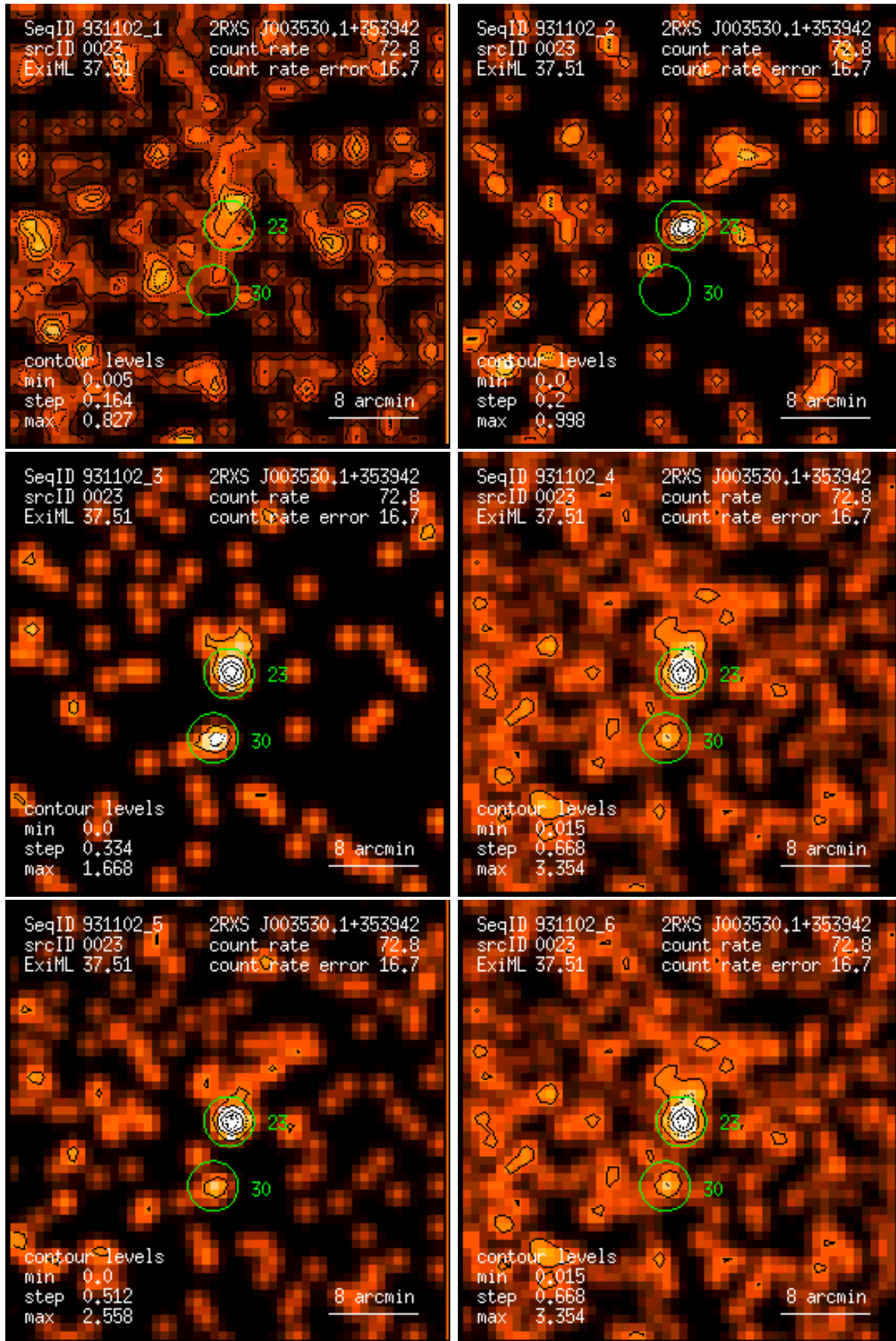
Figure 23: RASS 931102: detection 0023: band rate images, Gaussian filter: (1) PSPC channels 11 – 41, (2) 52 – 90, (3) 91 – 201, (4) 11 – 235, (5) 52 – 201, (6) 11 – 201. Broad band rates in counts/ks. Band rate contour levels in counts/ks/arcmin 2 .
