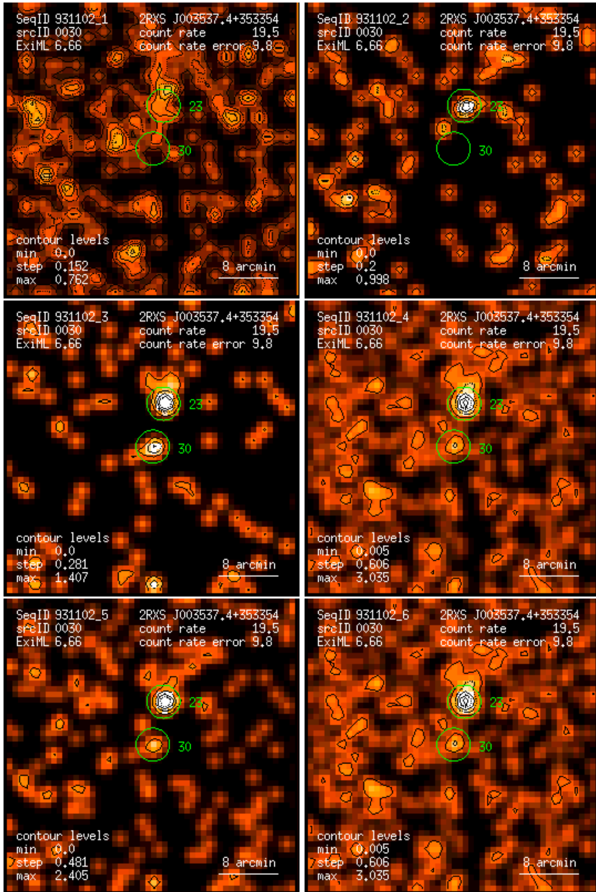
Figure 30: RASS 931102: detection 0030: band rate images, Gaussian filter: (1) PSPC channels 11 – 41, (2) 52 – 90, (3) 91 – 201, (4) 11 – 235, (5) 52 – 201, (6) 11 – 201. Broad band rates in counts/ks. Band rate contour levels in counts/ks/arcmin 2 .
