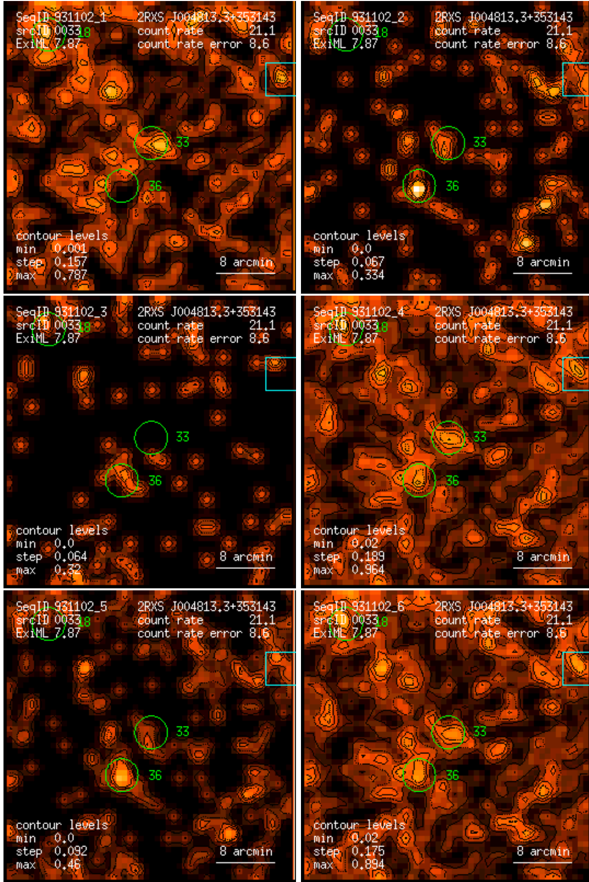
Figure 33: RASS 931102: detection 0033: band rate images, Gaussian filter: (1) PSPC channels 11 – 41, (2) 52 – 90, (3) 91 – 201, (4) 11 – 235, (5) 52 – 201, (6) 11 – 201. Broad band rates in counts/ks. Band rate contour levels in counts/ks/arcmin 2 .
