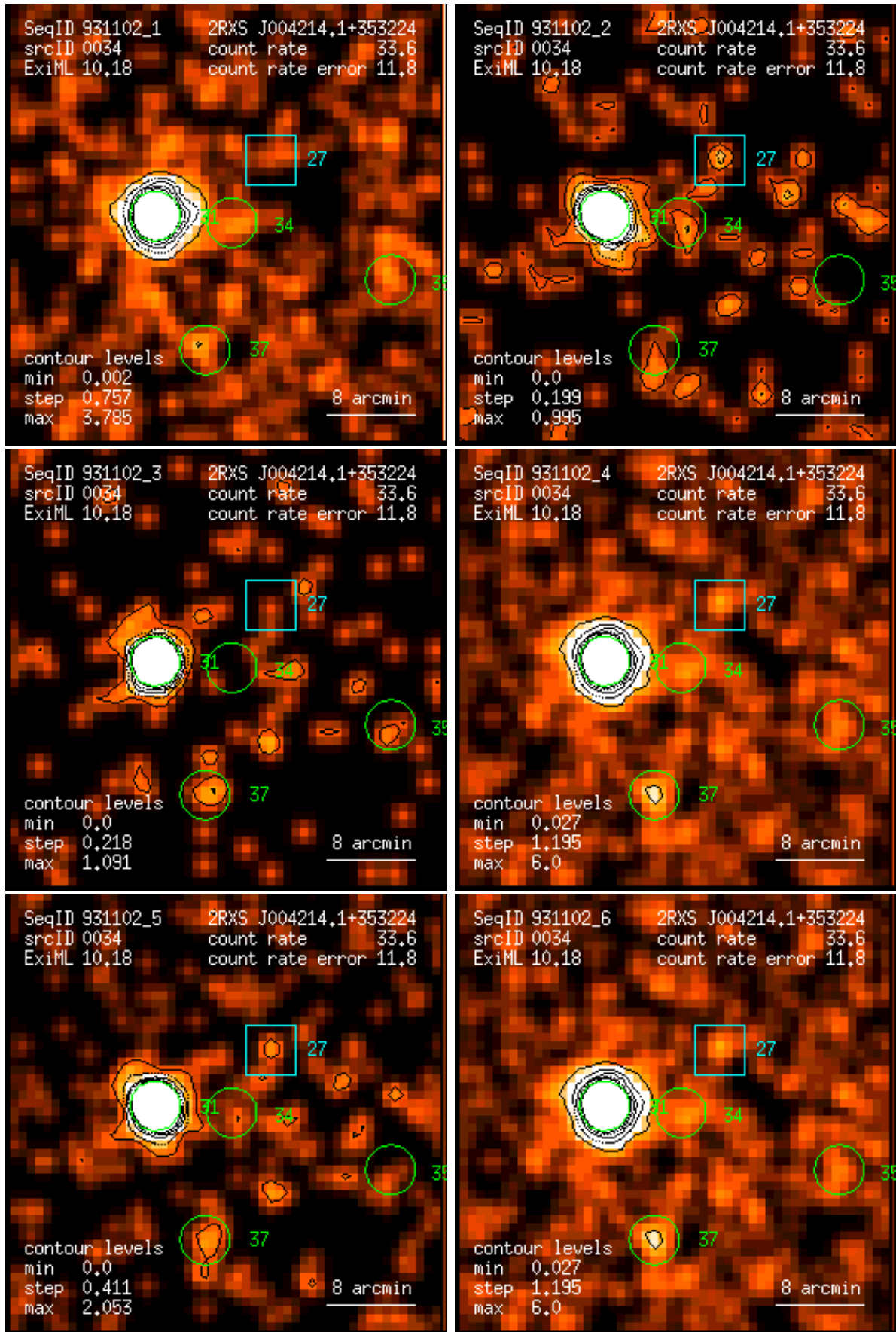
Figure 34: RASS 931102: detection 0034: band rate images, Gaussian filter: (1) PSPC channels 11 – 41, (2) 52 – 90, (3) 91 – 201, (4) 11 – 235, (5) 52 – 201, (6) 11 – 201. Broad band rates in counts/ks. Band rate contour levels in counts/ks/arcmin 2 .
