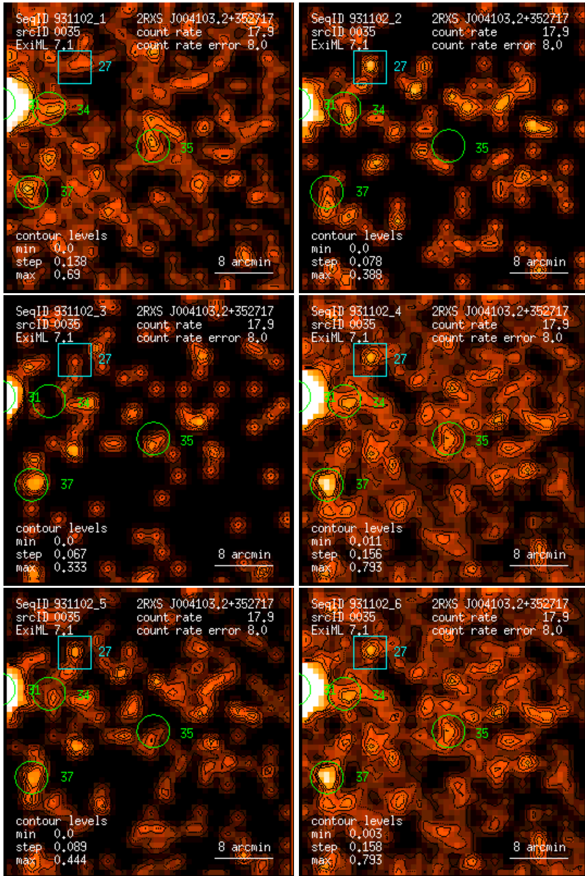
Figure 35: RASS 931102: detection 0035: band rate images, Gaussian filter: (1) PSPC channels 11 – 41, (2) 52 – 90, (3) 91 – 201, (4) 11 – 235, (5) 52 – 201, (6) 11 – 201. Broad band rates in counts/ks. Band rate contour levels in counts/ks/arcmin 2 .
