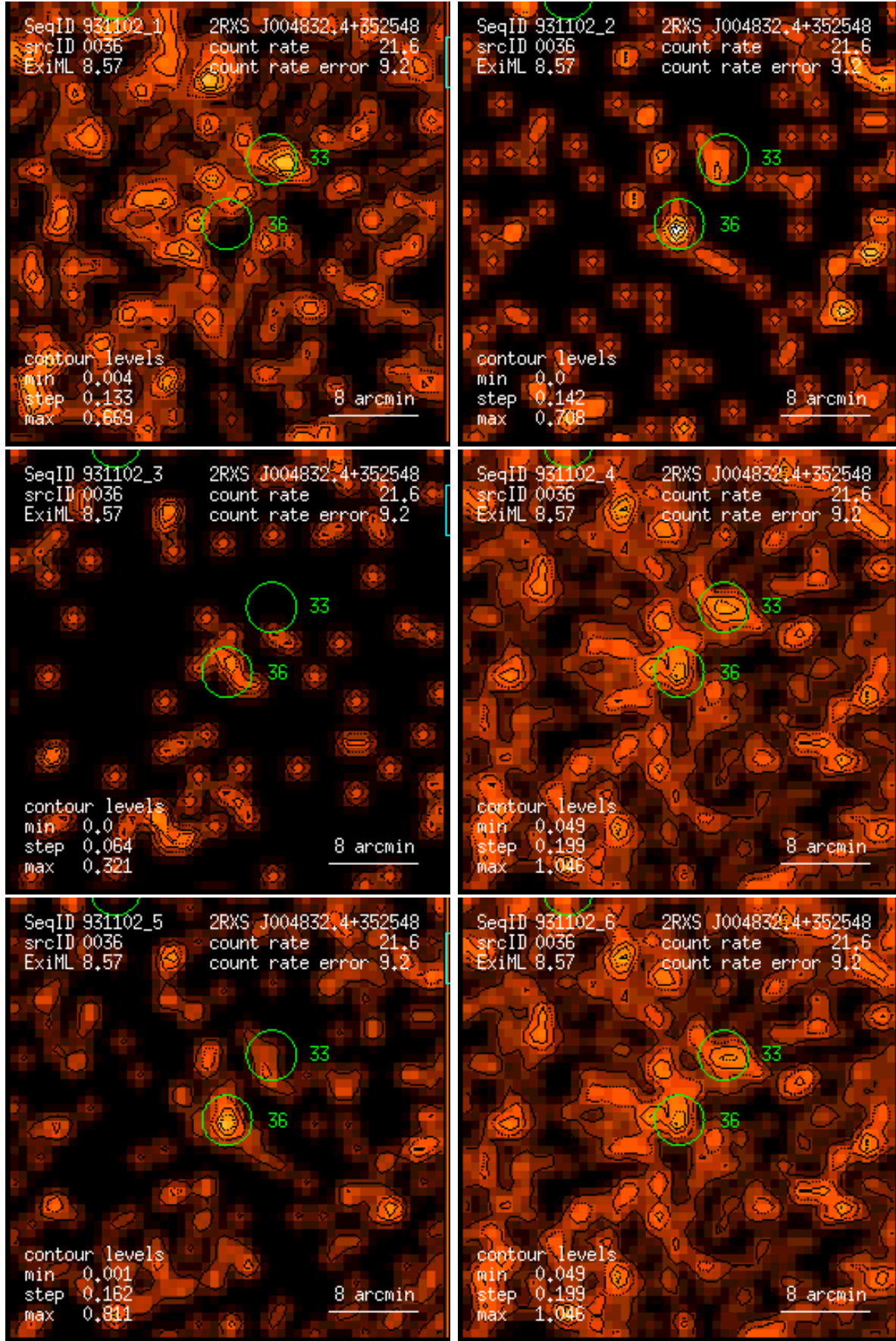
Figure 36: RASS 931102: detection 0036: band rate images, Gaussian filter: (1) PSPC channels 11 – 41, (2) 52 – 90, (3) 91 – 201, (4) 11 – 235, (5) 52 – 201, (6) 11 – 201. Broad band rates in counts/ks. Band rate contour levels in counts/ks/arcmin 2 .
