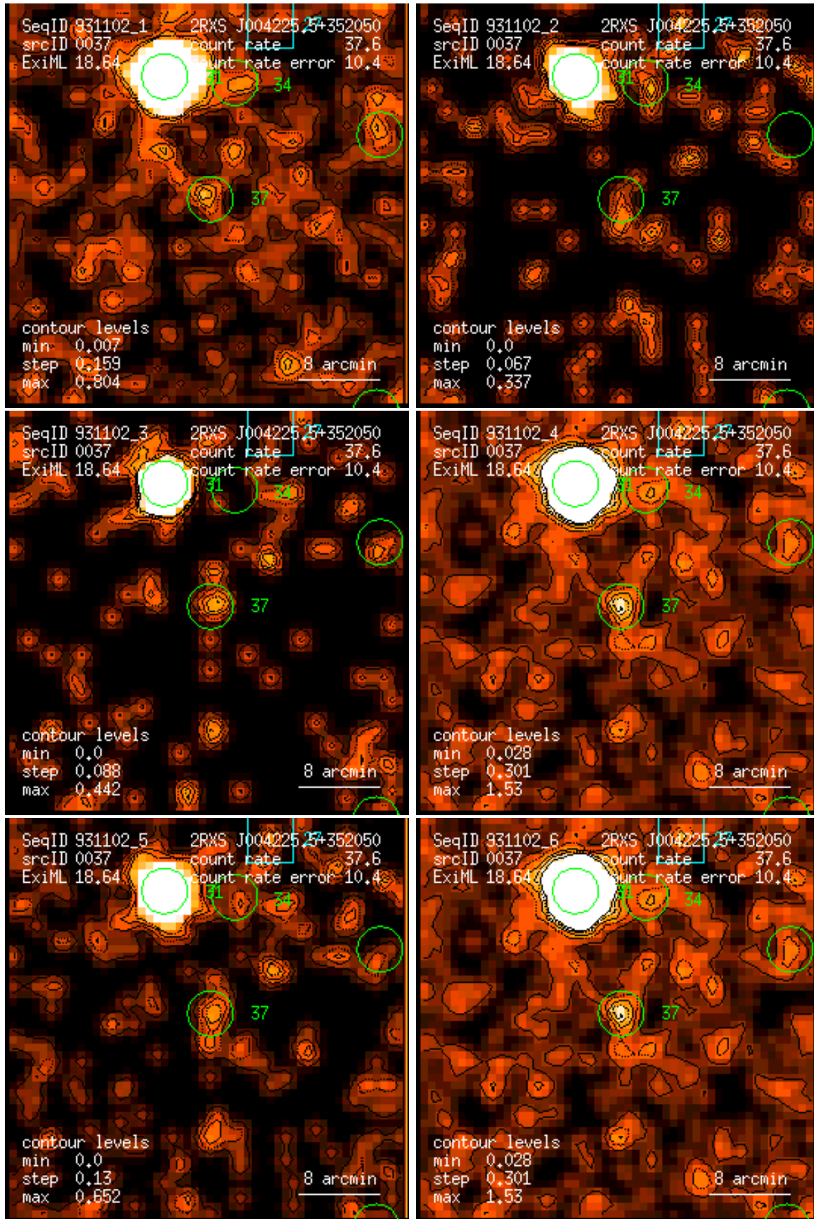
Figure 37: RASS 931102: detection 0037: band rate images, Gaussian filter: (1) PSPC channels 11 – 41, (2) 52 – 90, (3) 91 – 201, (4) 11 – 235, (5) 52 – 201, (6) 11 – 201. Broad band rates in counts/ks. Band rate contour levels in counts/ks/arcmin 2 .
