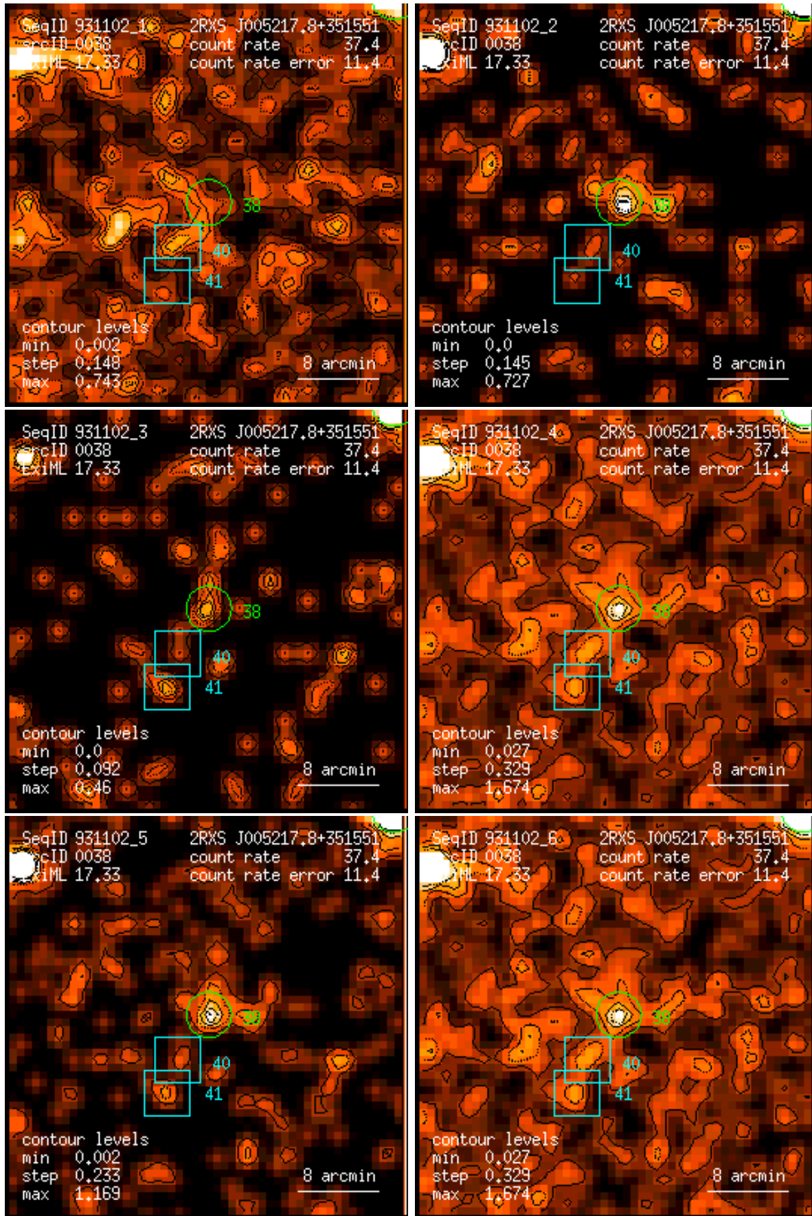
Figure 38: RASS 931102: detection 0038: band rate images, Gaussian filter: (1) PSPC channels 11 – 41, (2) 52 – 90, (3) 91 – 201, (4) 11 – 235, (5) 52 – 201, (6) 11 – 201. Broad band rates in counts/ks. Band rate contour levels in counts/ks/arcmin 2 .
