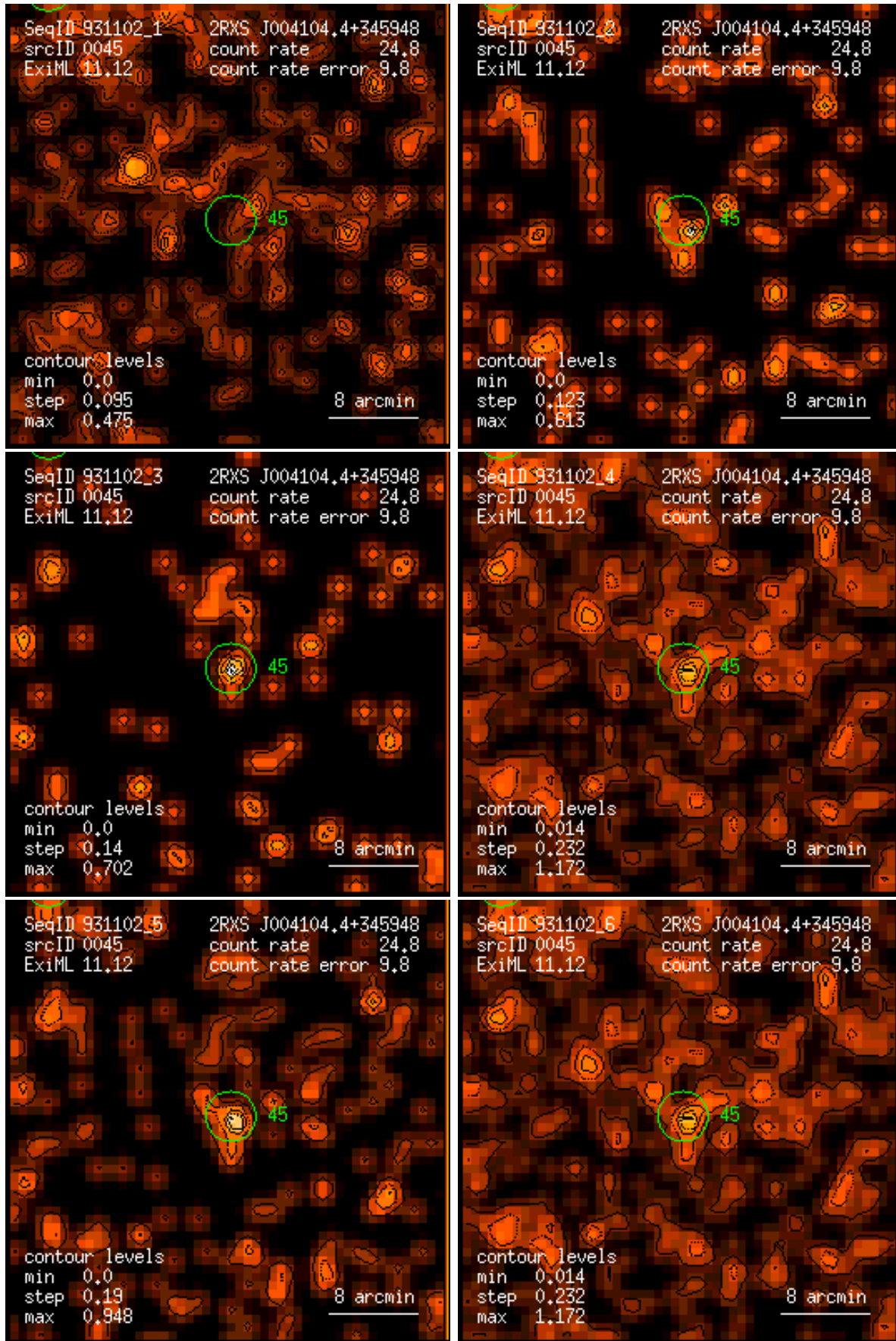
Figure 45: RASS 931102: detection 0045: band rate images, Gaussian filter: (1) PSPC channels 11 – 41, (2) 52 – 90, (3) 91 – 201, (4) 11 – 235, (5) 52 – 201, (6) 11 – 201. Broad band rates in counts/ks. Band rate contour levels in counts/ks/arcmin 2 .
