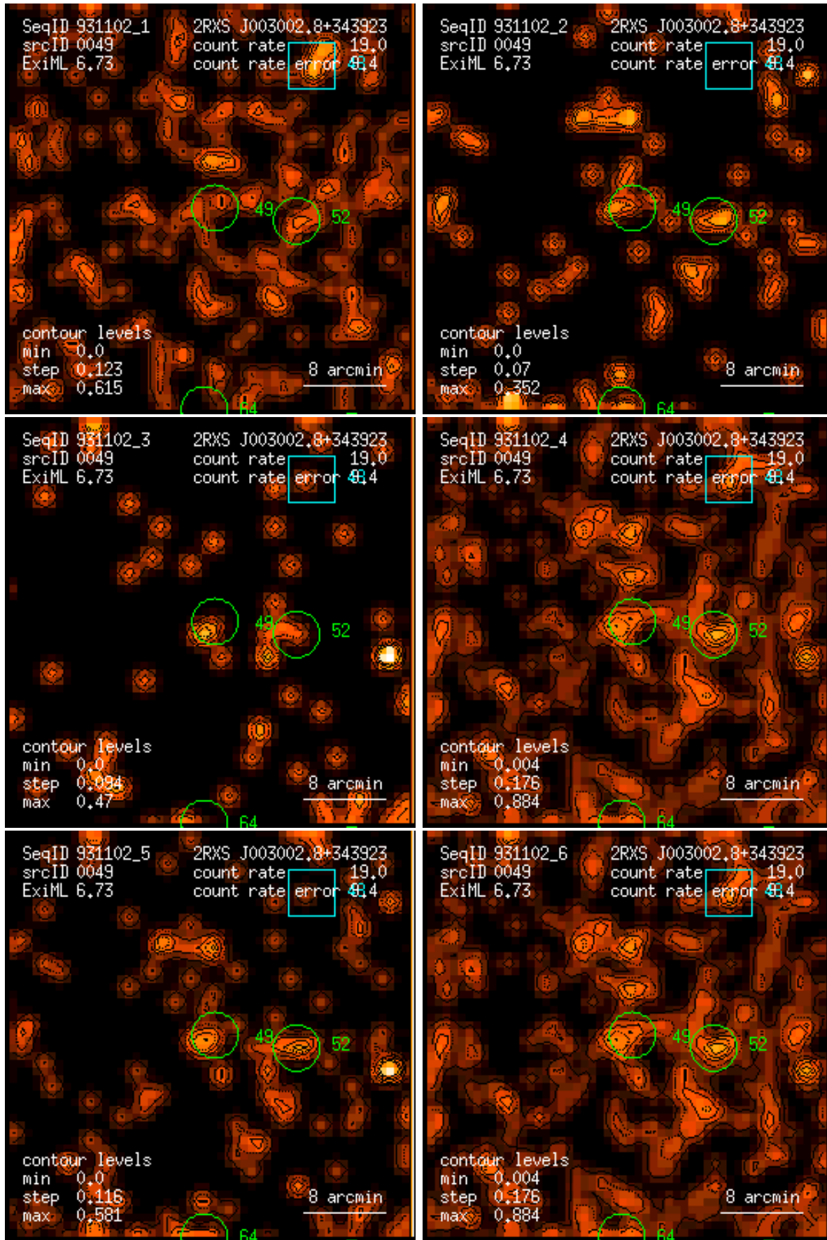
Figure 49: RASS 931102: detection 0049: band rate images, Gaussian filter: (1) PSPC channels 11 – 41, (2) 52 – 90, (3) 91 – 201, (4) 11 – 235, (5) 52 – 201, (6) 11 – 201. Broad band rates in counts/ks. Band rate contour levels in counts/ks/arcmin 2 .
