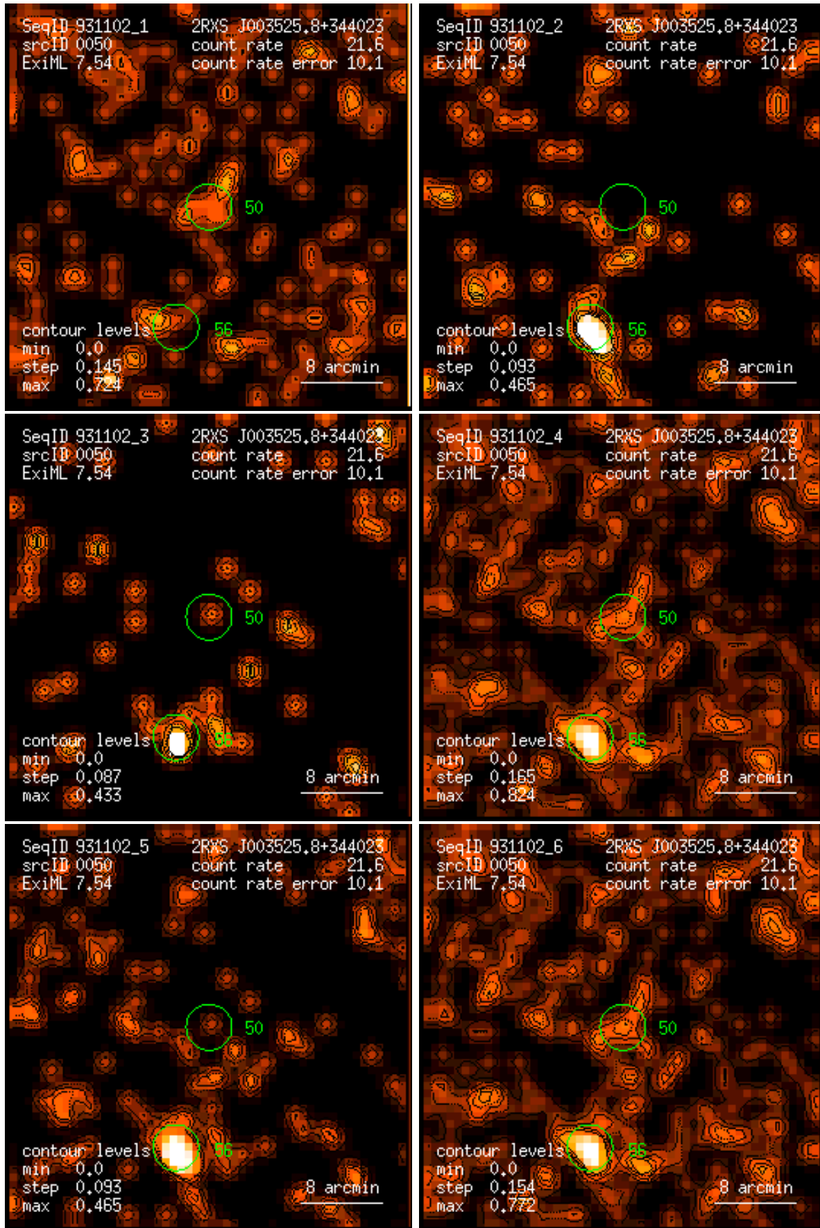
Figure 50: RASS 931102: detection 0050: band rate images, Gaussian filter: (1) PSPC channels 11 – 41, (2) 52 – 90, (3) 91 – 201, (4) 11 – 235, (5) 52 – 201, (6) 11 – 201. Broad band rates in counts/ks. Band rate contour levels in counts/ks/arcmin 2 .
