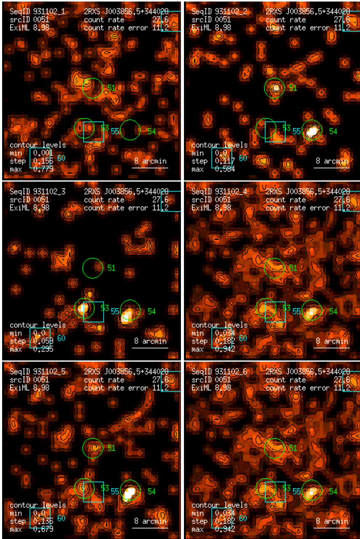
Figure 51: RASS 931102: detection 0051: band rate images, Gaussian filter: (1) PSPC channels 11 – 41, (2) 52 – 90, (3) 91 – 201, (4) 11 – 235, (5) 52 – 201, (6) 11 – 201. Broad band rates in counts/ks. Band rate contour levels in counts/ks/arcmin 2 .
