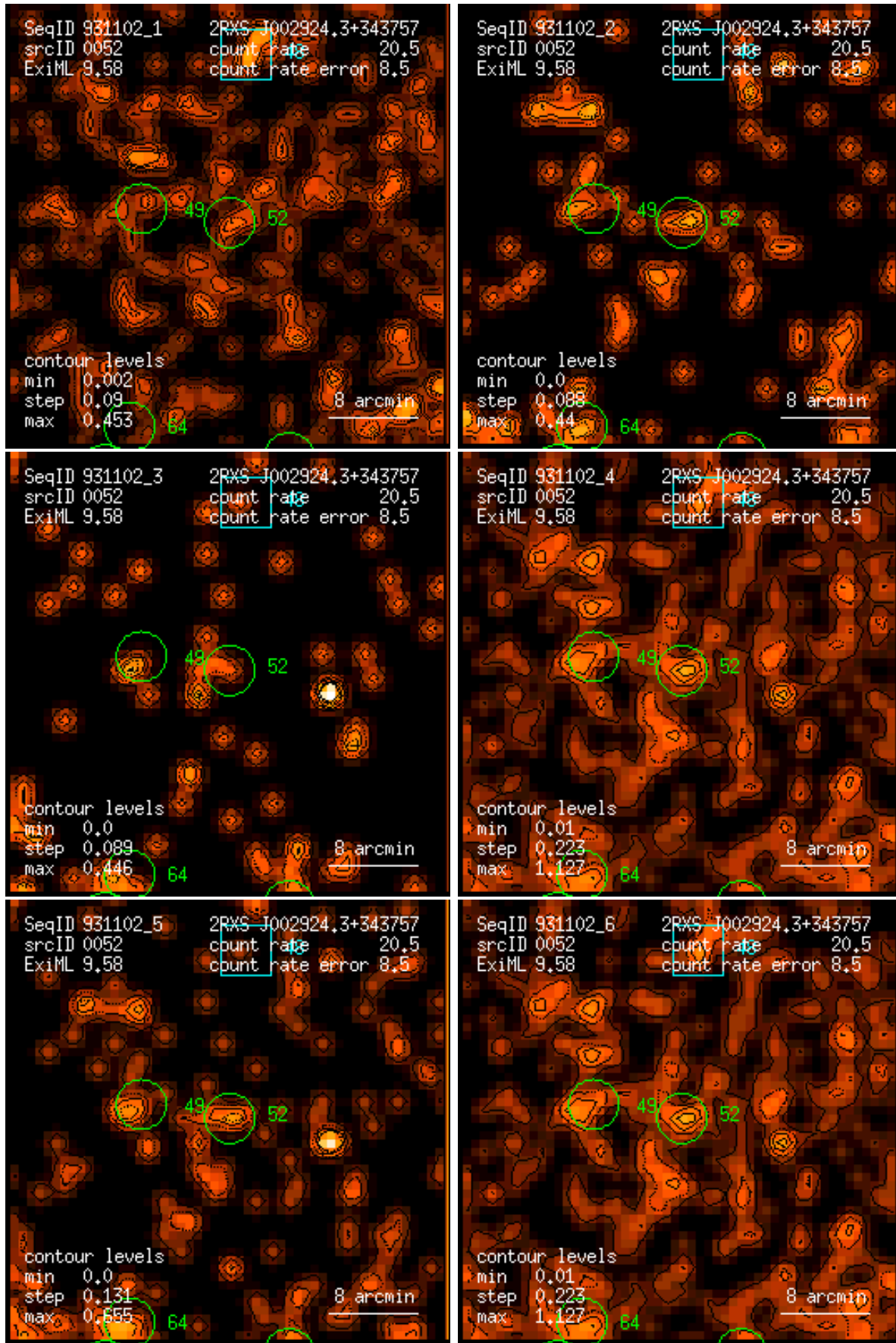
Figure 52: RASS 931102: detection 0052: band rate images, Gaussian filter: (1) PSPC channels 11 – 41, (2) 52 – 90, (3) 91 – 201, (4) 11 – 235, (5) 52 – 201, (6) 11 – 201. Broad band rates in counts/ks. Band rate contour levels in counts/ks/arcmin 2 .
