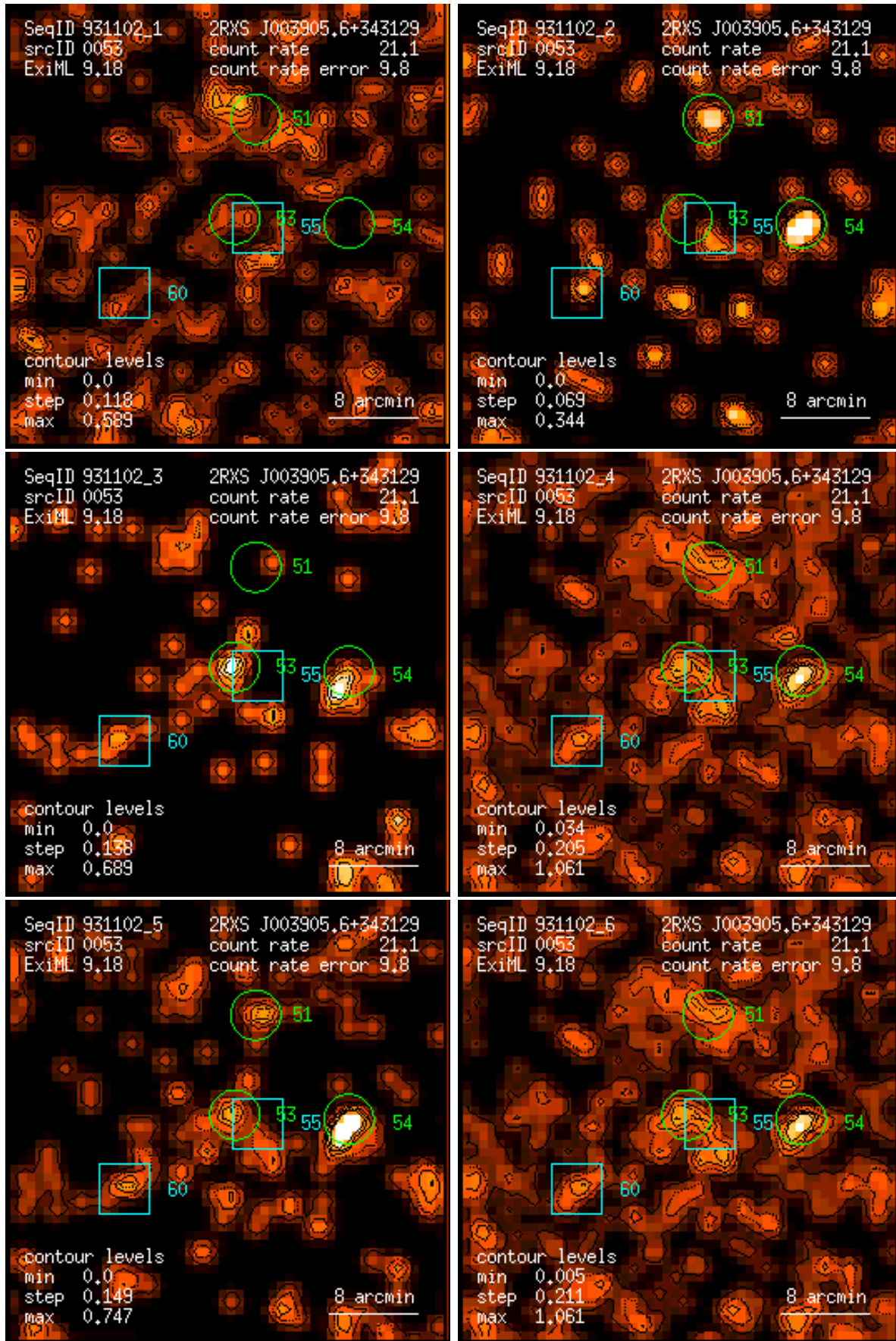
Figure 53: RASS 931102: detection 0053: band rate images, Gaussian filter: (1) PSPC channels 11 – 41, (2) 52 – 90, (3) 91 – 201, (4) 11 – 235, (5) 52 – 201, (6) 11 – 201. Broad band rates in counts/ks. Band rate contour levels in counts/ks/arcmin 2 .
