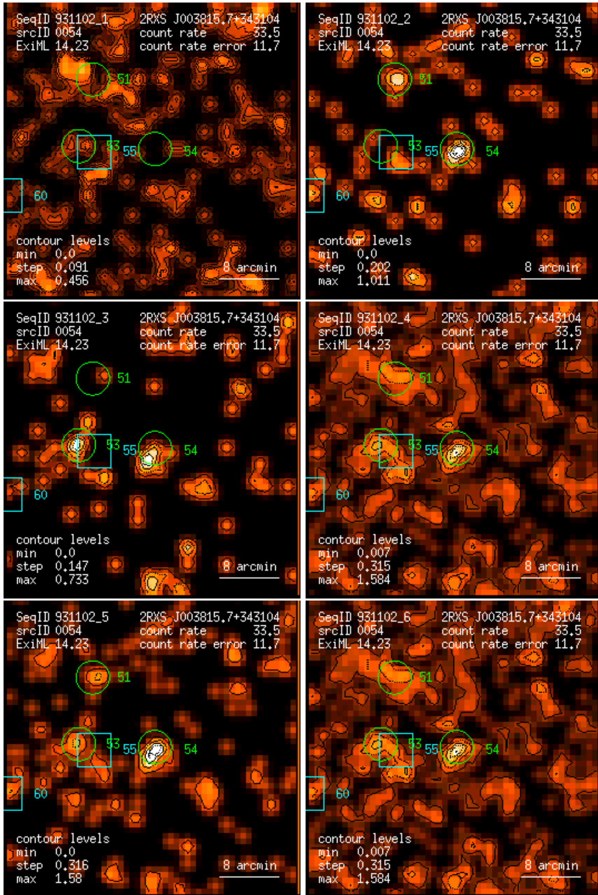
Figure 54: RASS 931102: detection 0054: band rate images, Gaussian filter: (1) PSPC channels 11 – 41, (2) 52 – 90, (3) 91 – 201, (4) 11 – 235, (5) 52 – 201, (6) 11 – 201. Broad band rates in counts/ks. Band rate contour levels in counts/ks/arcmin 2 .
