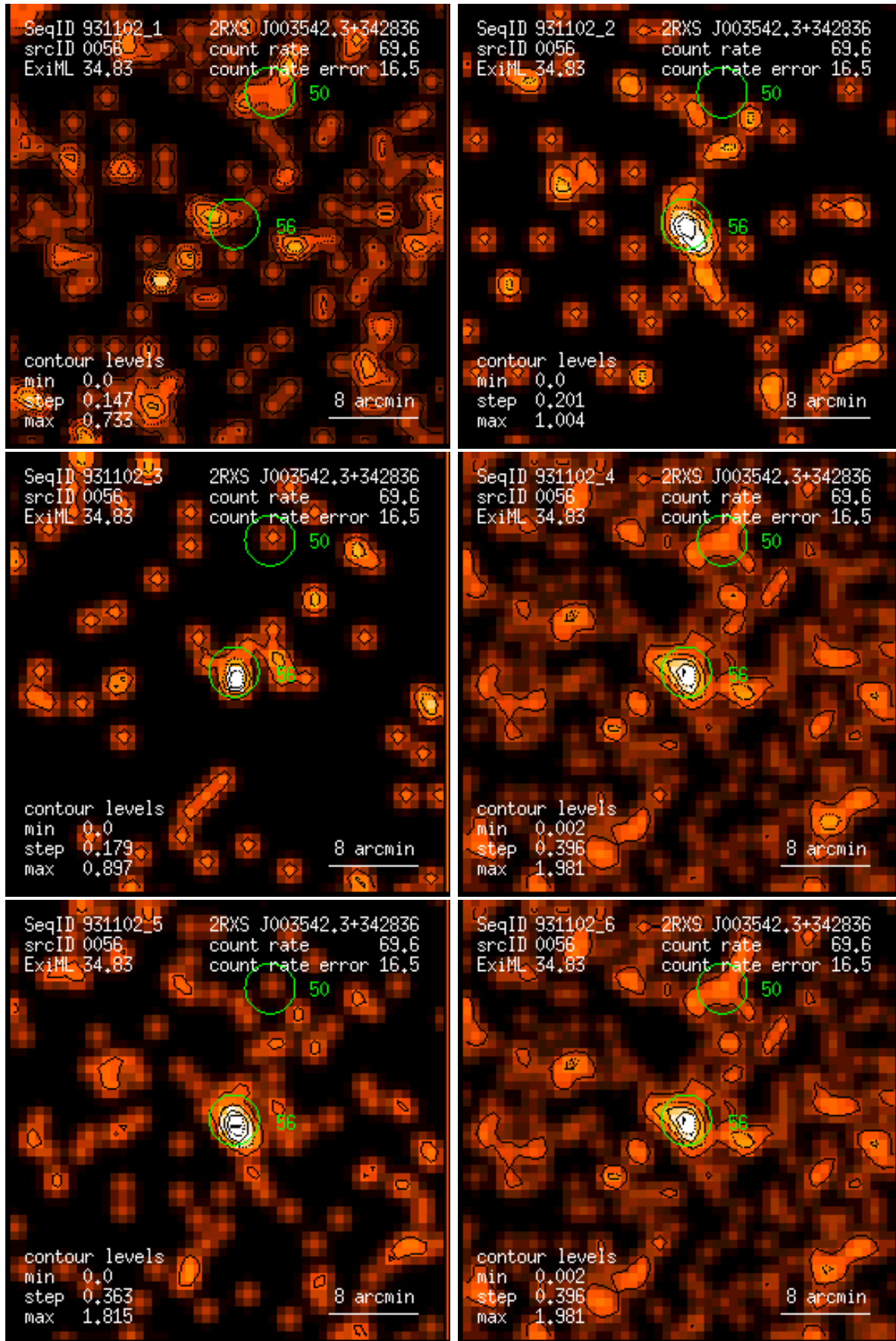
Figure 56: RASS 931102: detection 0056: band rate images, Gaussian filter: (1) PSPC channels 11 – 41, (2) 52 – 90, (3) 91 – 201, (4) 11 – 235, (5) 52 – 201, (6) 11 – 201. Broad band rates in counts/ks. Band rate contour levels in counts/ks/arcmin 2 .
