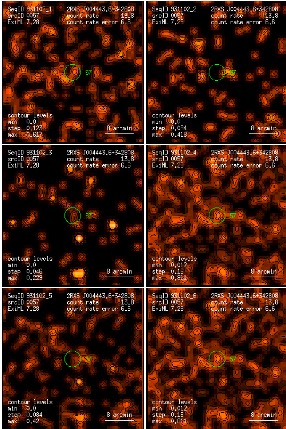
Figure 57: RASS 931102: detection 0057: band rate images, Gaussian filter: (1) PSPC channels 11 – 41, (2) 52 – 90, (3) 91 – 201, (4) 11 – 235, (5) 52 – 201, (6) 11 – 201. Broad band rates in counts/ks. Band rate contour levels in counts/ks/arcmin 2 .
