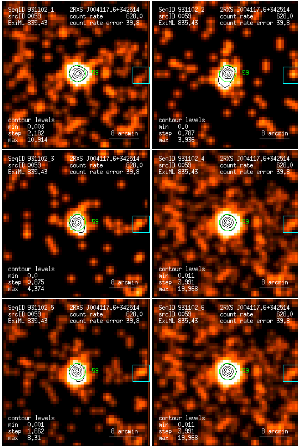
Figure 59: RASS 931102: detection 0059: band rate images, Gaussian filter: (1) PSPC channels 11 – 41, (2) 52 – 90, (3) 91 – 201, (4) 11 – 235, (5) 52 – 201, (6) 11 – 201. Broad band rates in counts/ks. Band rate contour levels in counts/ks/arcmin 2 .
