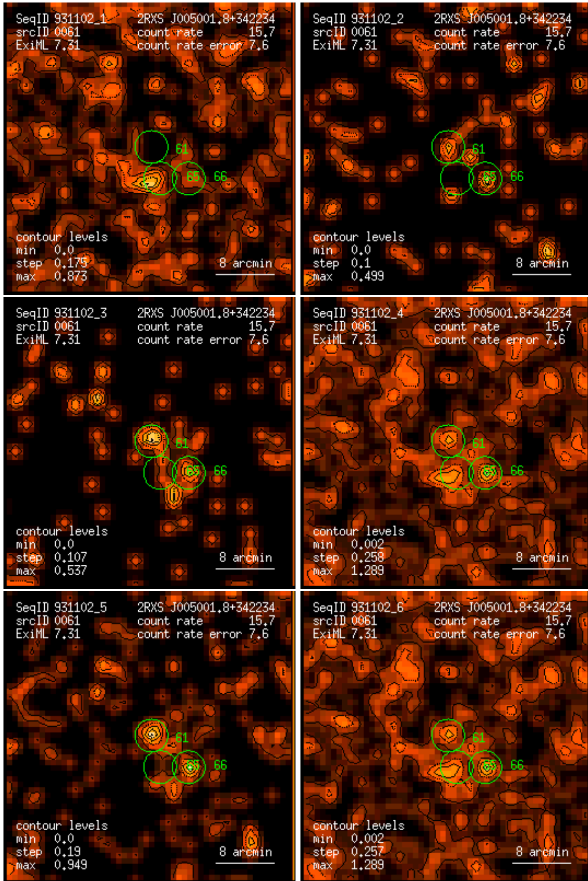
Figure 61: RASS 931102: detection 0061: band rate images, Gaussian filter: (1) PSPC channels 11 – 41, (2) 52 – 90, (3) 91 – 201, (4) 11 – 235, (5) 52 – 201, (6) 11 – 201. Broad band rates in counts/ks. Band rate contour levels in counts/ks/arcmin 2 .
