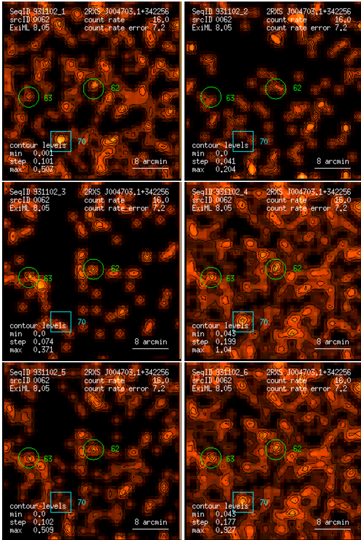
Figure 62: RASS 931102: detection 0062: band rate images, Gaussian filter: (1) PSPC channels 11 – 41, (2) 52 – 90, (3) 91 – 201, (4) 11 – 235, (5) 52 – 201, (6) 11 – 201. Broad band rates in counts/ks. Band rate contour levels in counts/ks/arcmin 2 .
