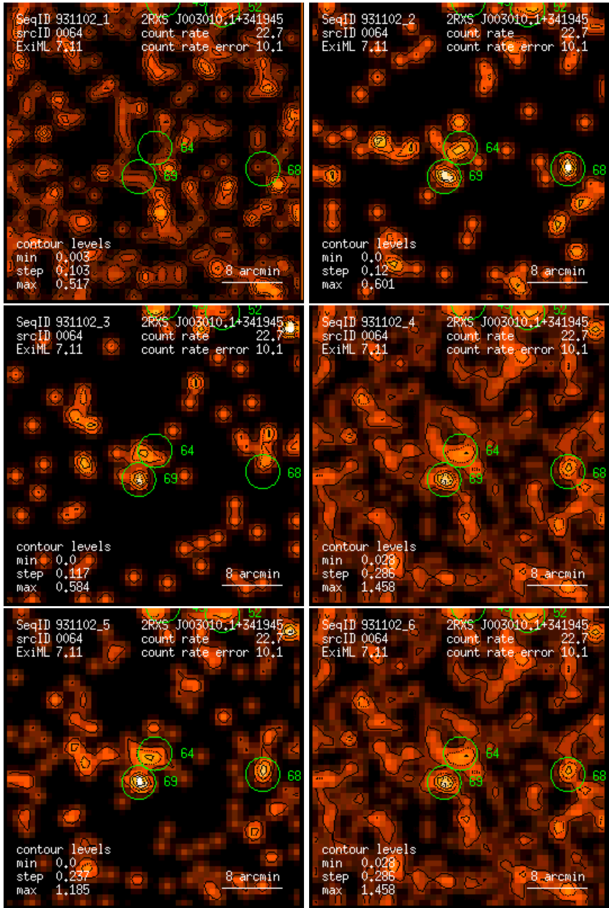
Figure 64: RASS 931102: detection 0064: band rate images, Gaussian filter: (1) PSPC channels 11 – 41, (2) 52 – 90, (3) 91 – 201, (4) 11 – 235, (5) 52 – 201, (6) 11 – 201. Broad band rates in counts/ks. Band rate contour levels in counts/ks/arcmin 2 .
