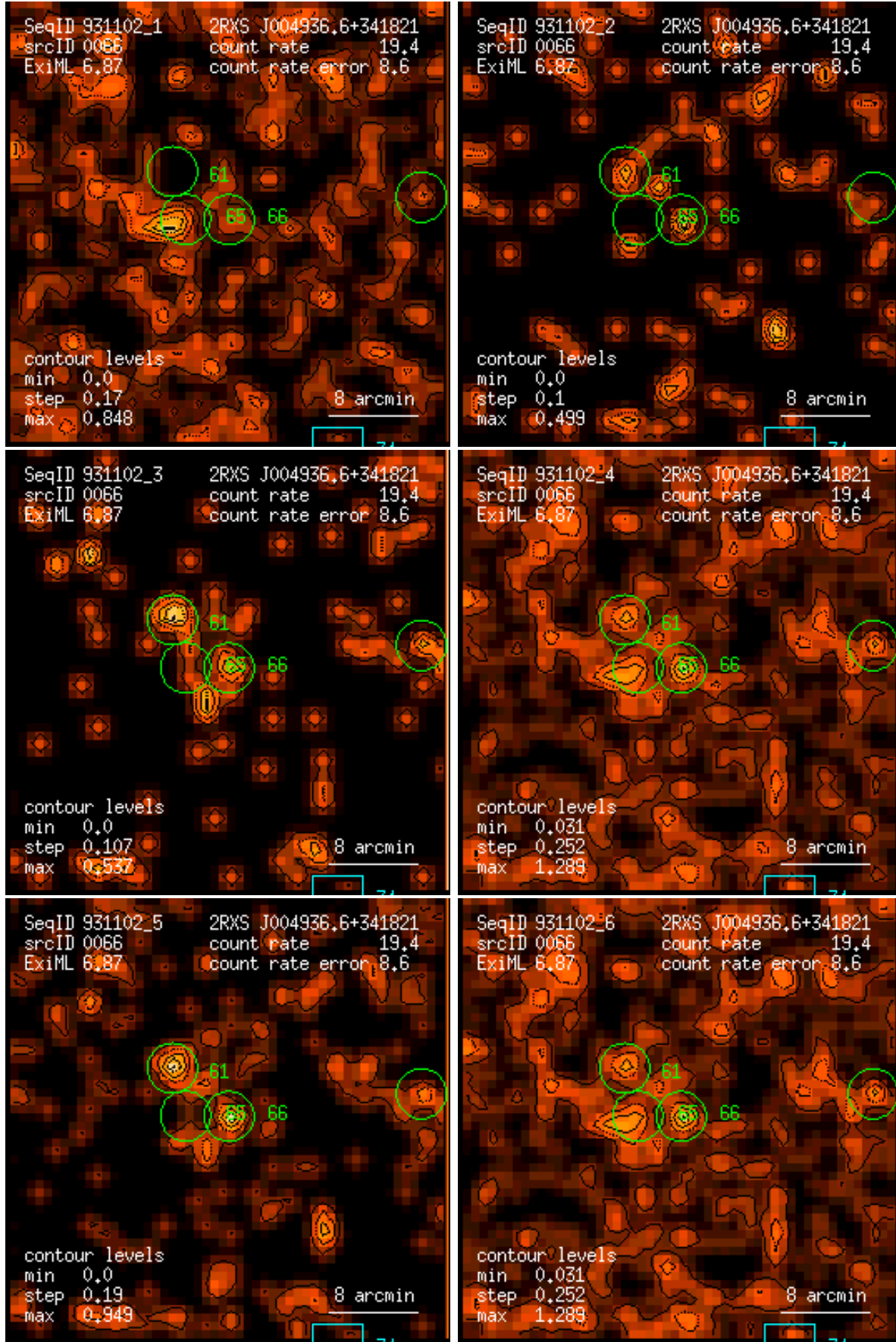
Figure 66: RASS 931102: detection 0066: band rate images, Gaussian filter: (1) PSPC channels 11 – 41, (2) 52 – 90, (3) 91 – 201, (4) 11 – 235, (5) 52 – 201, (6) 11 – 201. Broad band rates in counts/ks. Band rate contour levels in counts/ks/arcmin 2 .
