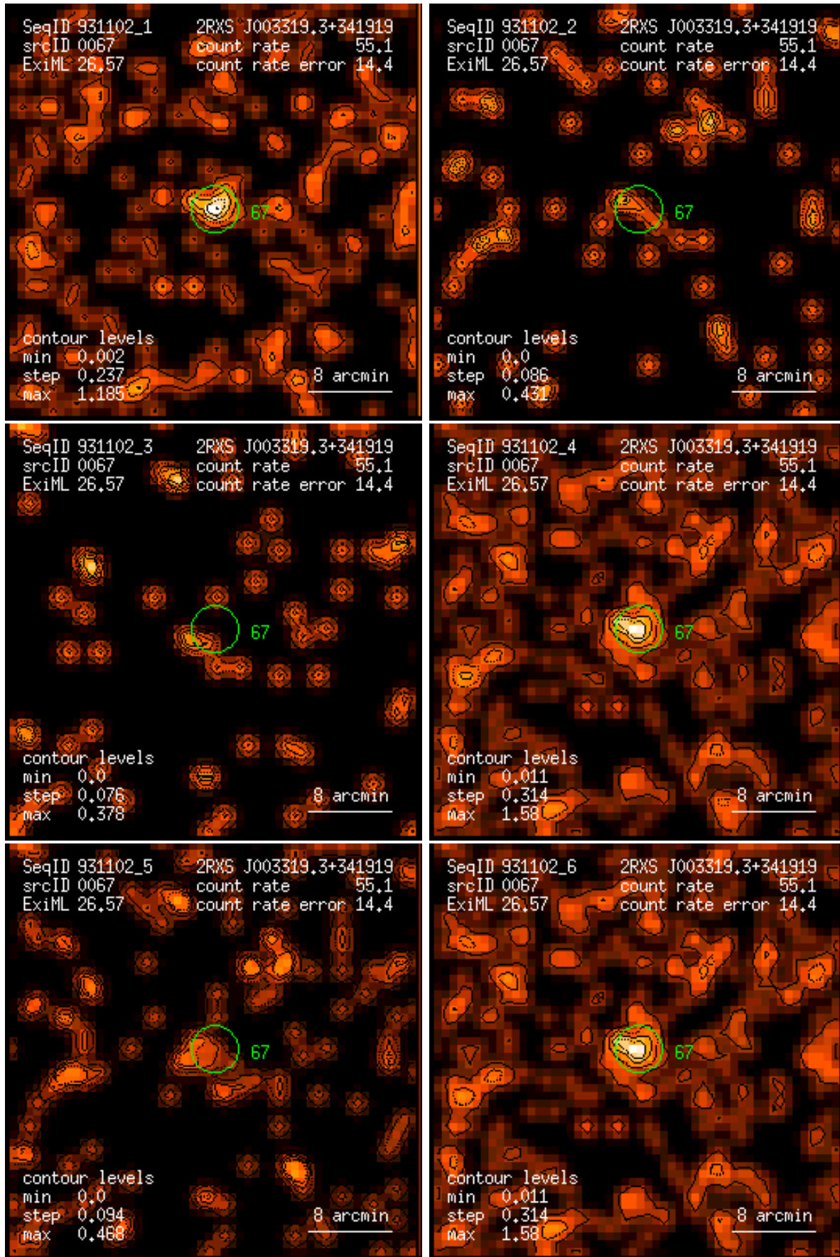
Figure 67: RASS 931102: detection 0067: band rate images, Gaussian filter: (1) PSPC channels 11 – 41, (2) 52 – 90, (3) 91 – 201, (4) 11 – 235, (5) 52 – 201, (6) 11 – 201. Broad band rates in counts/ks. Band rate contour levels in counts/ks/arcmin 2 .
