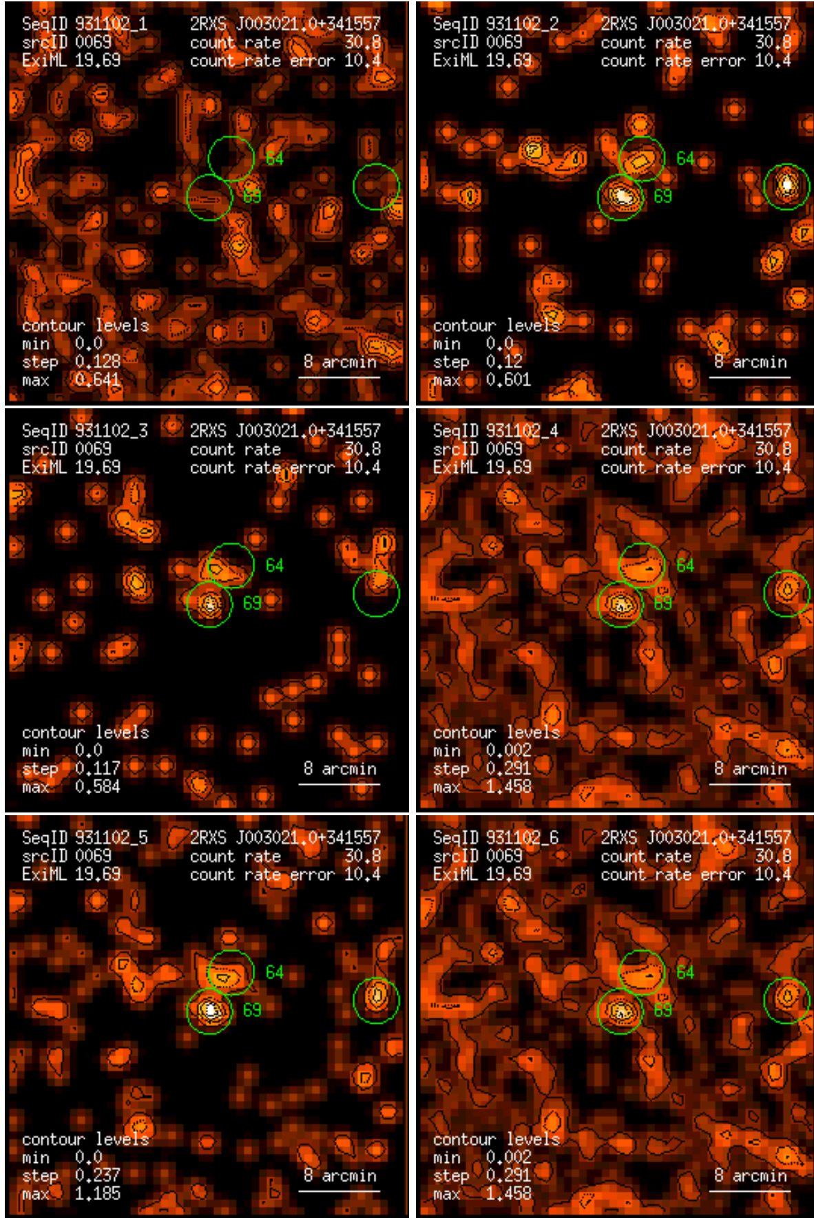
Figure 69: RASS 931102: detection 0069: band rate images, Gaussian filter: (1) PSPC channels 11 – 41, (2) 52 – 90, (3) 91 – 201, (4) 11 – 235, (5) 52 – 201, (6) 11 – 201. Broad band rates in counts/ks. Band rate contour levels in counts/ks/arcmin 2 .
