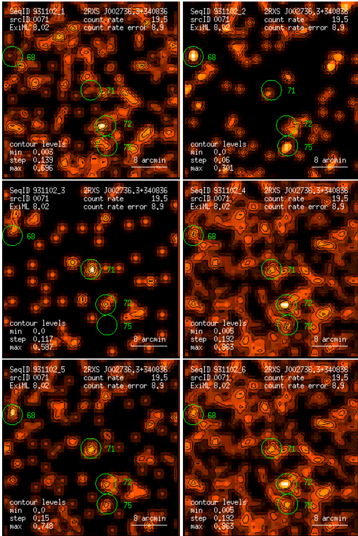
Figure 71: RASS 931102: detection 0071: band rate images, Gaussian filter: (1) PSPC channels 11 – 41, (2) 52 – 90, (3) 91 – 201, (4) 11 – 235, (5) 52 – 201, (6) 11 – 201. Broad band rates in counts/ks. Band rate contour levels in counts/ks/arcmin 2 .
