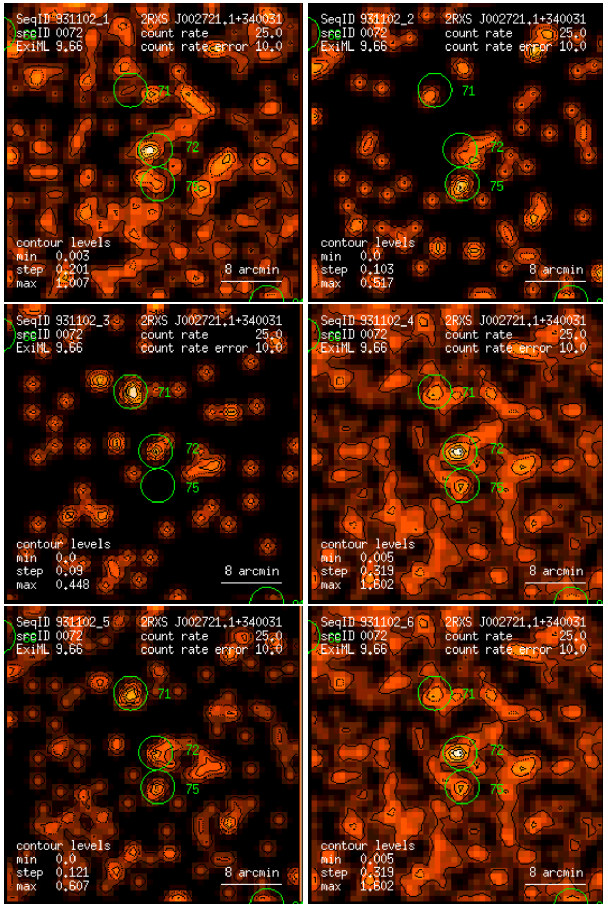
Figure 72: RASS 931102: detection 0072: band rate images, Gaussian filter: (1) PSPC channels 11 – 41, (2) 52 – 90, (3) 91 – 201, (4) 11 – 235, (5) 52 – 201, (6) 11 – 201. Broad band rates in counts/ks. Band rate contour levels in counts/ks/arcmin 2 .
