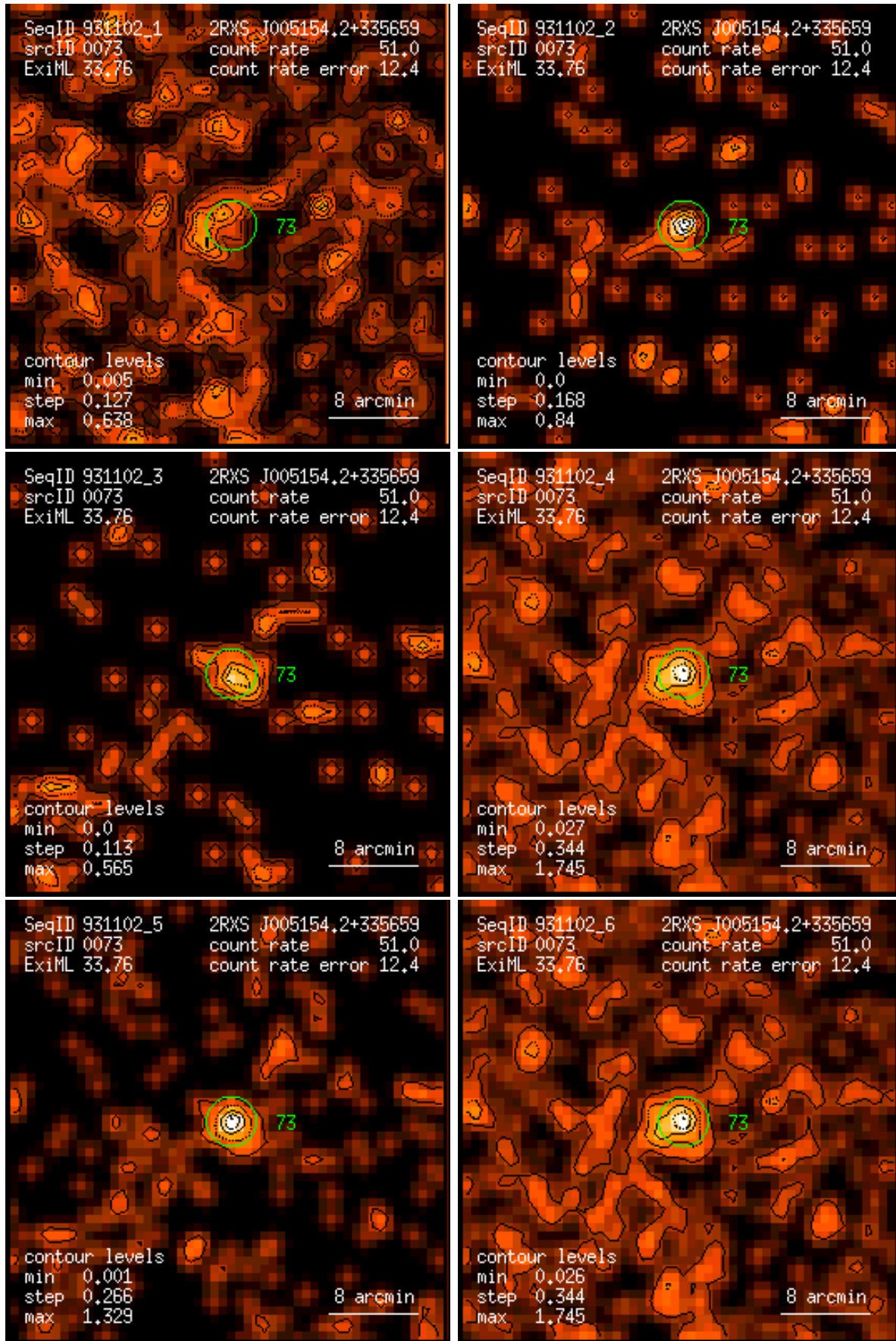
Figure 73: RASS 931102: detection 0073: band rate images, Gaussian filter: (1) PSPC channels 11 – 41, (2) 52 – 90, (3) 91 – 201, (4) 11 – 235, (5) 52 – 201, (6) 11 – 201. Broad band rates in counts/ks. Band rate contour levels in counts/ks/arcmin 2 .
