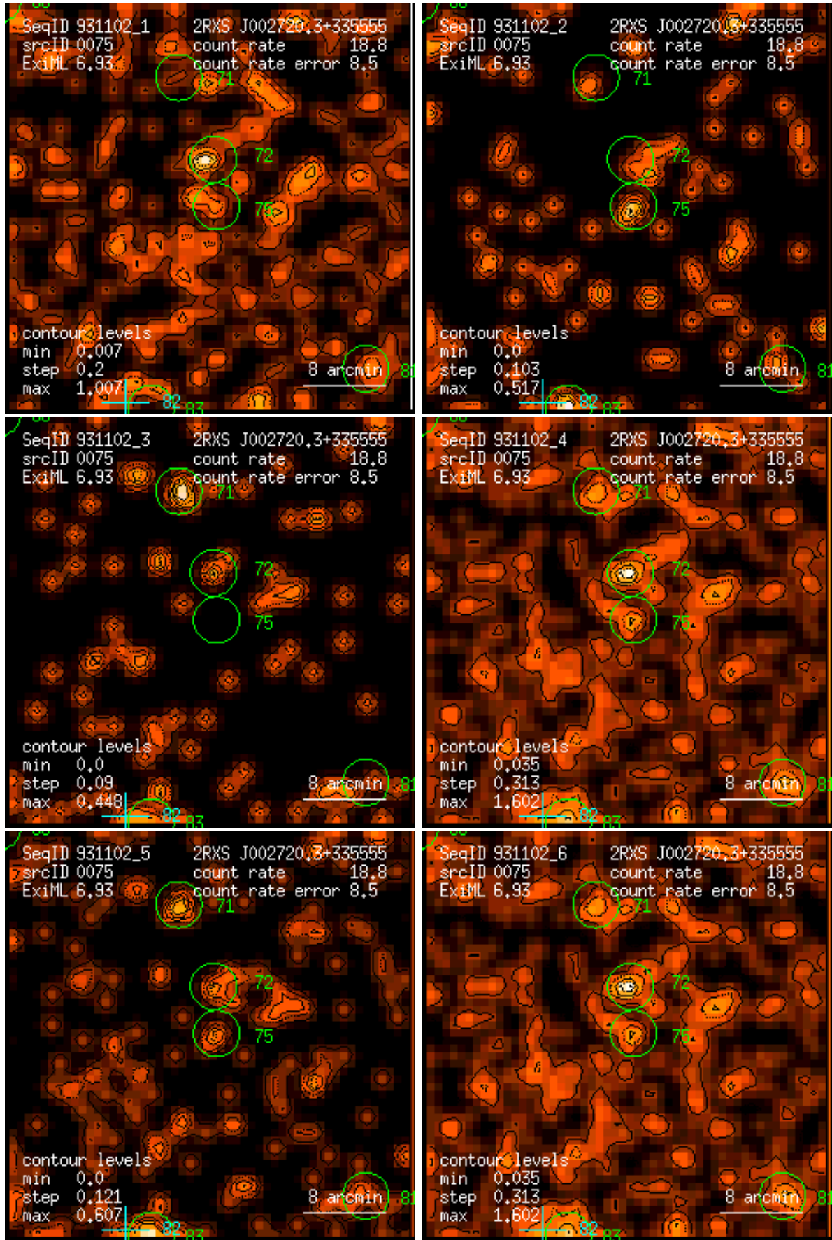
Figure 75: RASS 931102: detection 0075: band rate images, Gaussian filter: (1) PSPC channels 11 – 41, (2) 52 – 90, (3) 91 – 201, (4) 11 – 235, (5) 52 – 201, (6) 11 – 201. Broad band rates in counts/ks. Band rate contour levels in counts/ks/arcmin 2 .
