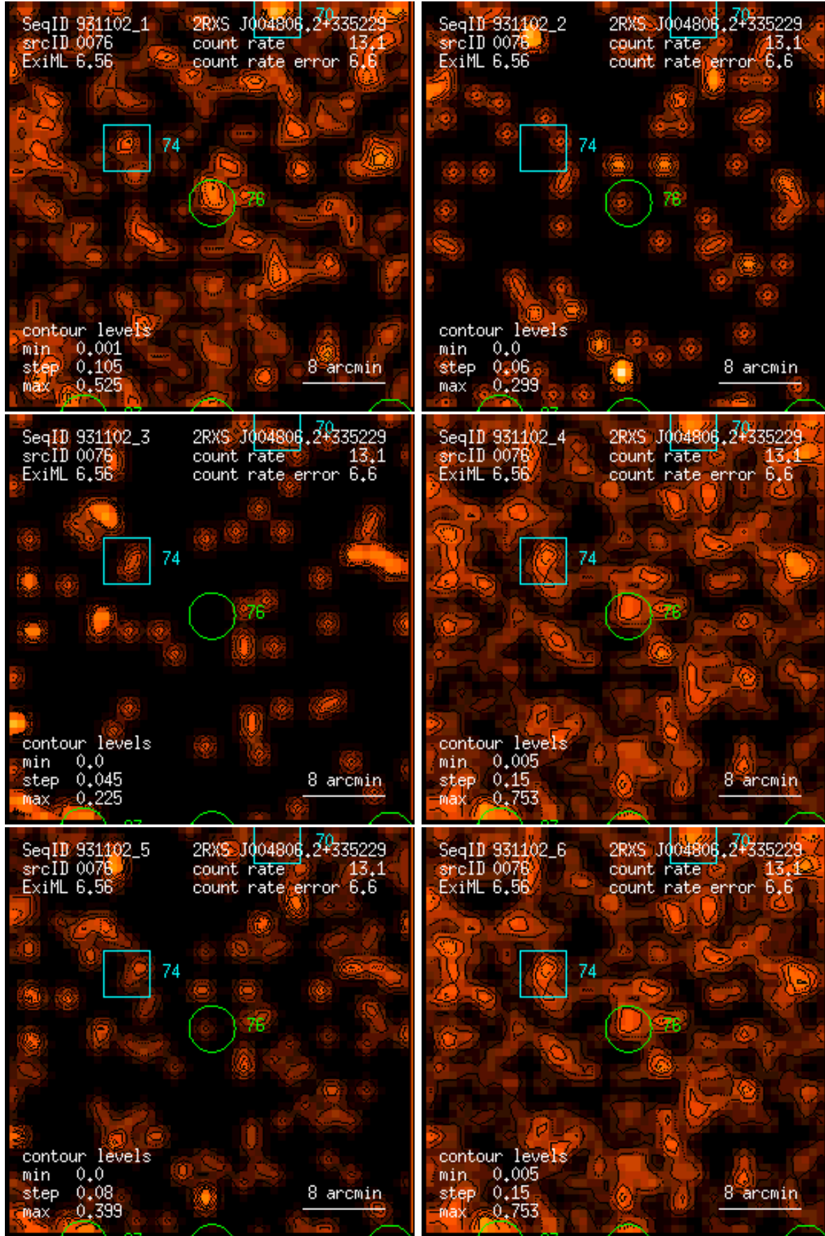
Figure 76: RASS 931102: detection 0076: band rate images, Gaussian filter: (1) PSPC channels 11 – 41, (2) 52 – 90, (3) 91 – 201, (4) 11 – 235, (5) 52 – 201, (6) 11 – 201. Broad band rates in counts/ks. Band rate contour levels in counts/ks/arcmin 2 .
