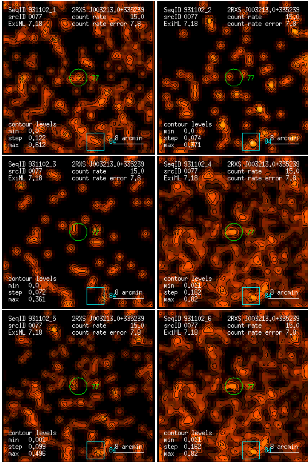
Figure 77: RASS 931102: detection 0077: band rate images, Gaussian filter: (1) PSPC channels 11 – 41, (2) 52 – 90, (3) 91 – 201, (4) 11 – 235, (5) 52 – 201, (6) 11 – 201. Broad band rates in counts/ks. Band rate contour levels in counts/ks/arcmin 2 .
