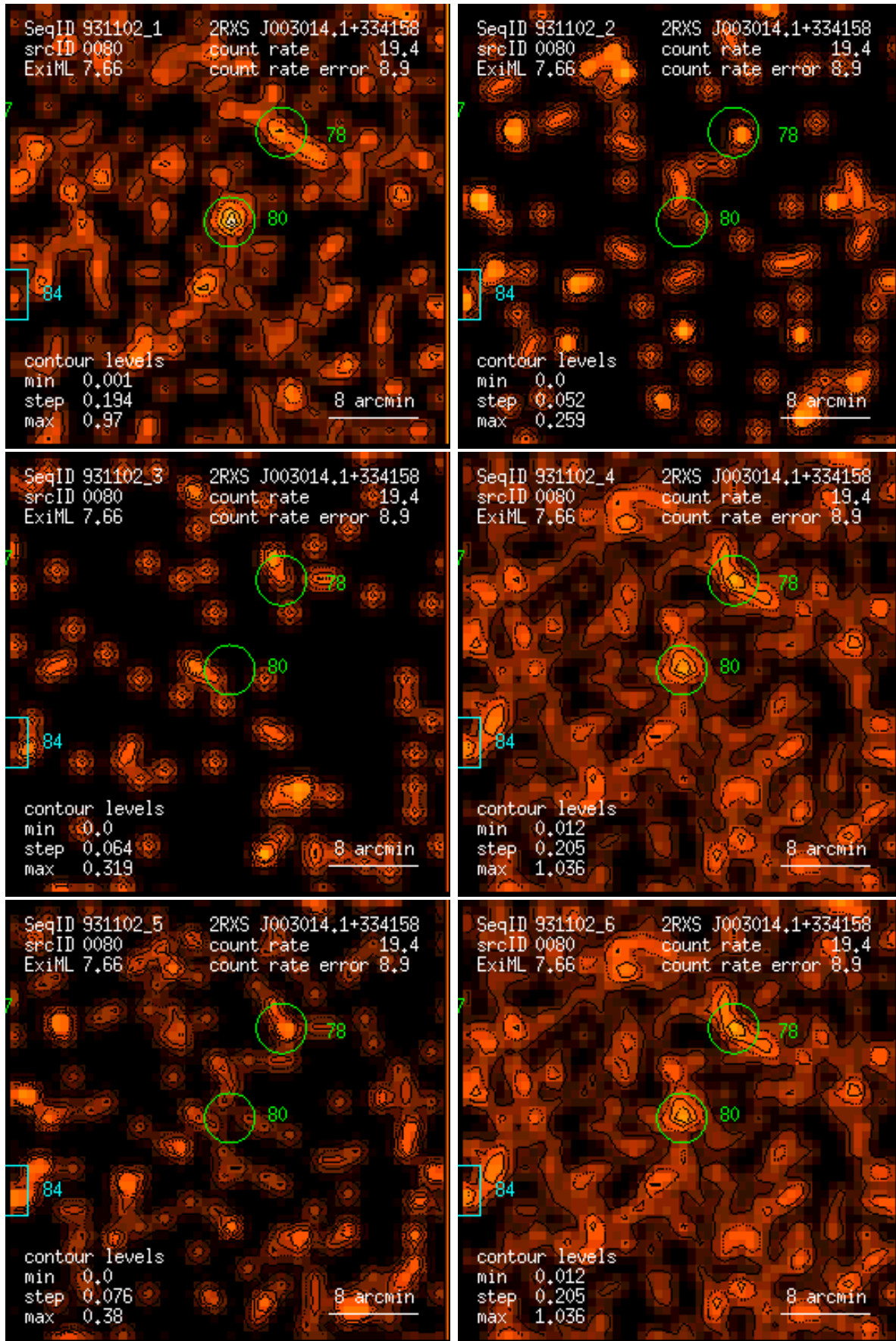
Figure 80: RASS 931102: detection 0080: band rate images, Gaussian filter: (1) PSPC channels 11 – 41, (2) 52 – 90, (3) 91 – 201, (4) 11 – 235, (5) 52 – 201, (6) 11 – 201. Broad band rates in counts/ks. Band rate contour levels in counts/ks/arcmin 2 .
